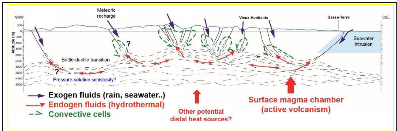
Figure 2: Understanding and questioning about the geothermal system as illustrated in the conceptual model of the deeper part of the Basse-Terre Island geothermal reservoir. Source: Garcia et al, 2021
