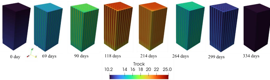
Figure 9: Temperature distribution of storage volume (15.975×13.845×36 m 3 ) at different times during the year. View is shown from the boundary of the storage volume.
