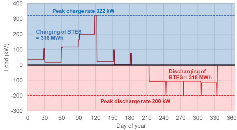
Figure 6: Applied heat load profile starting from 1 st April using half-day time intervals.
