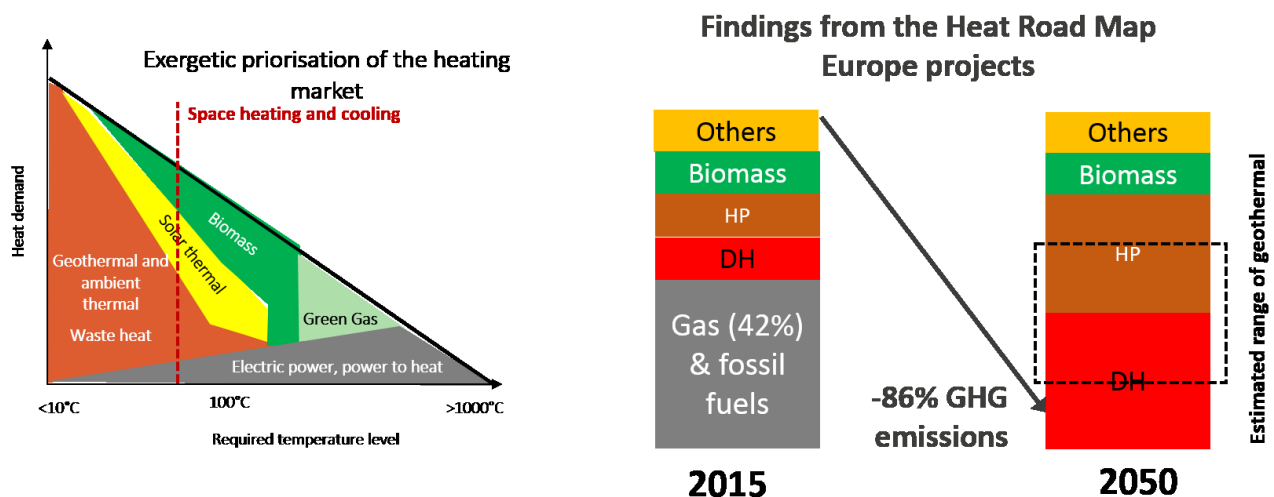
Figure 4: Basic concept of exergetic prioritization (left) and pathways towards the decarbonisation of the heating and cooling market in Europe based on figures published by the Heat Road Map Europe project ( https://heatroadmap.eu ).
