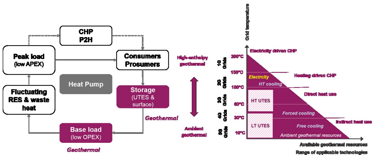
Figure 5: The possible role of geothermal energy into modern DHC network topologies (left) and the match between geothermal energy sources and heating networks of different generations (right).
