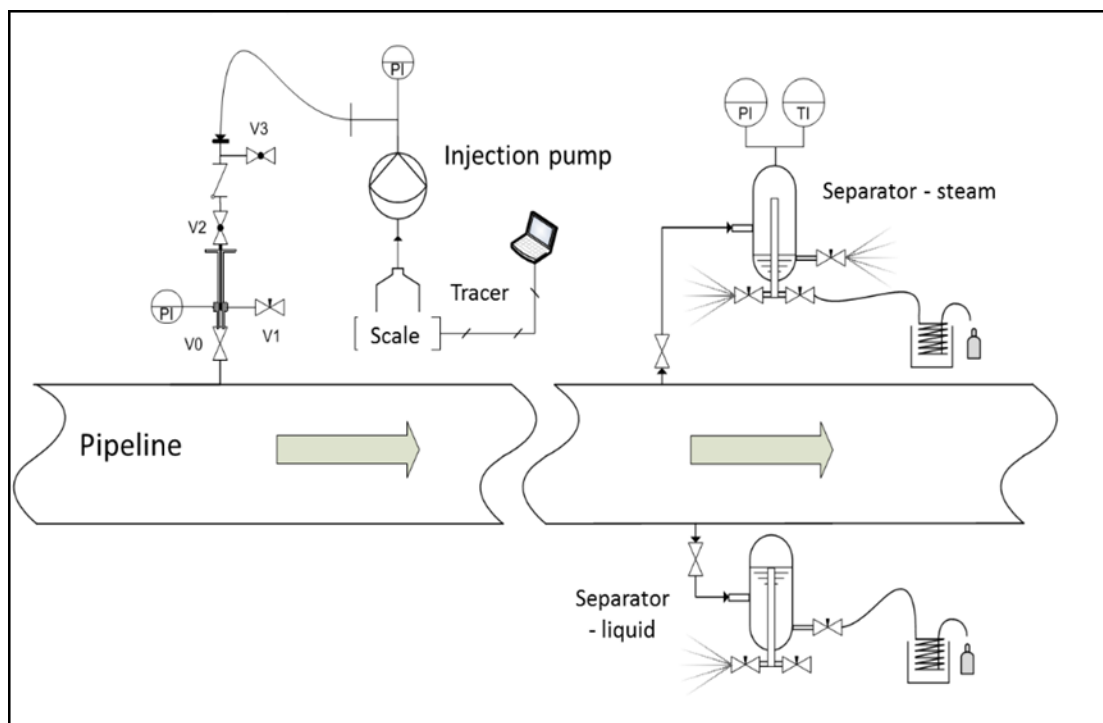
Figure 1: The figure above is a schematic impression showing injection equipment, tracer injection point, steam pipe, sampling point and sampling equipment.
