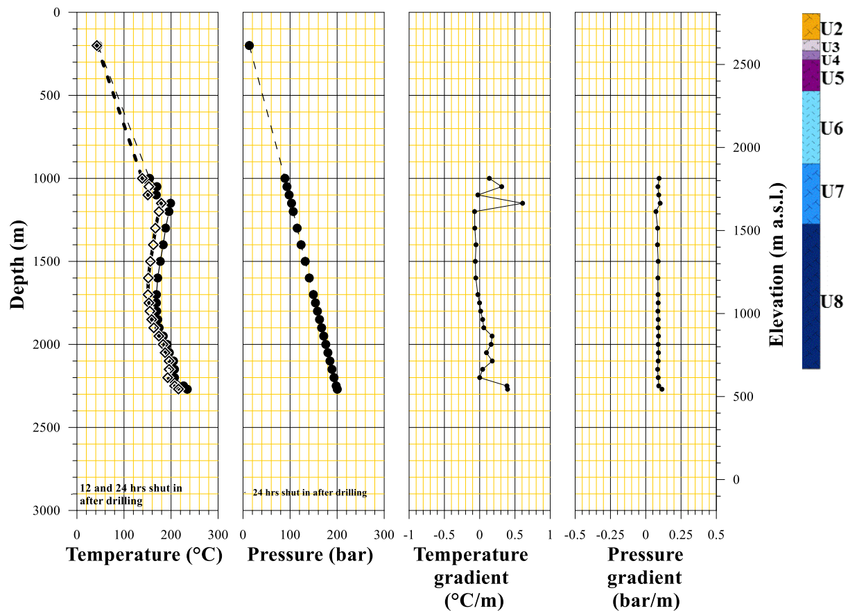
Figure 9: Profiles correlation of temperature, pressure, thermal gradient, pressure gradient and lithology of well H19, located at eastern block of LHGF north zone.
