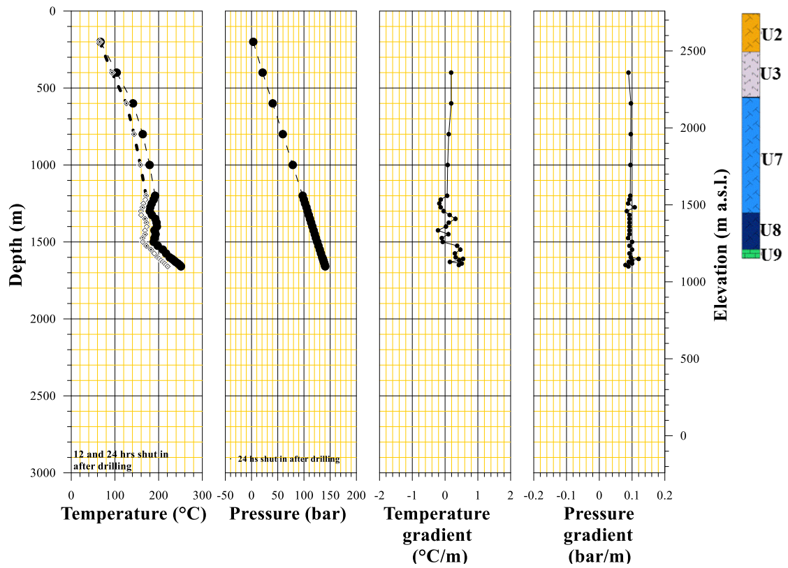
Figure 4: Profiles correlation of temperature, pressure, circulation losses, thermal gradient, pressure gradient and lithology of well H3.
