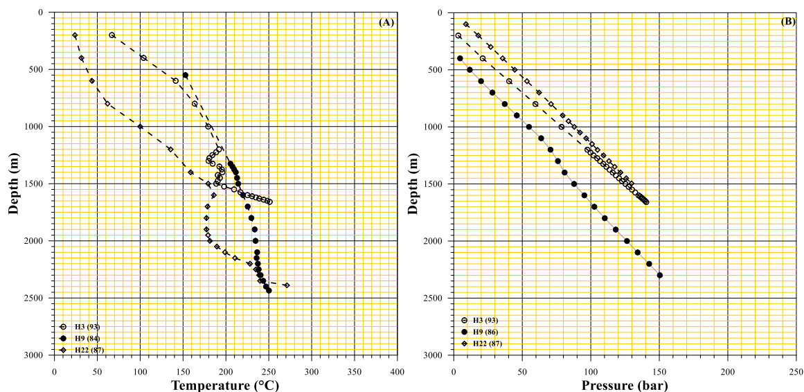
Figure 3: Temperature (A) and pressure (B) profiles of wells located at western block of north zone of LHGF, emerging the different behavior of H9 located more away of “Malpais” fault, respect to wells H3 and H22.
