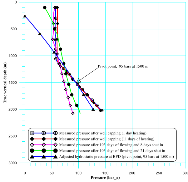
FIGURE 5: MW-20A pressure profiles
