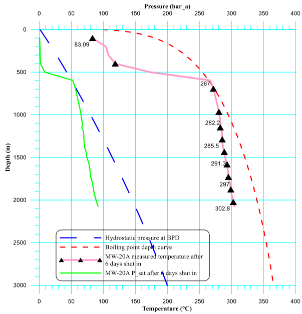
FIGURE 2: MW-20A temperature and pressure profiles after 103 days of flowing and six (6) days of shut-in
