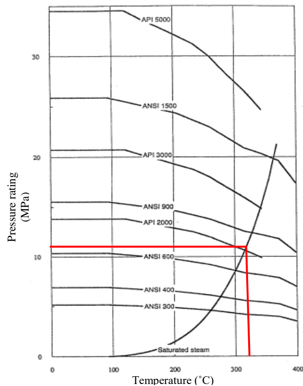
FIGURE 15: Wellhead working pressure de-rating for flanges and valves conforming to ANSI/ASME B16.5 and to API Spec 6A (New Zealand Standard,
