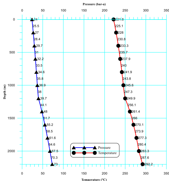
FIGURE 12: Flowing TP conditions in MW-20A
