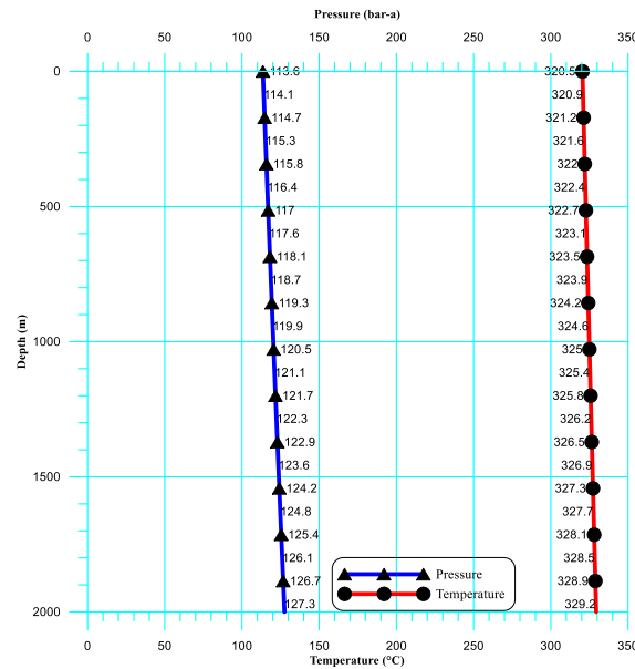
FIGURE 11: Steam conditions in MW-20A
