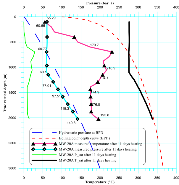
FIGURE 1: MW-20A temperature and pressure profiles 11 days after well capping
