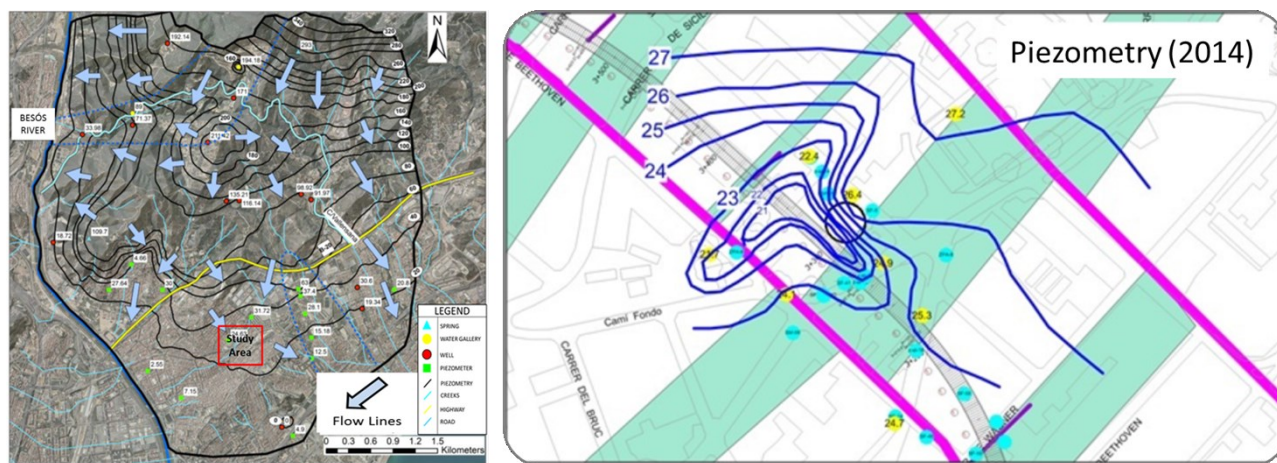
Figure 6. Left: Regional piezometric map (2016). Right: Study area piezometric map (2014)
