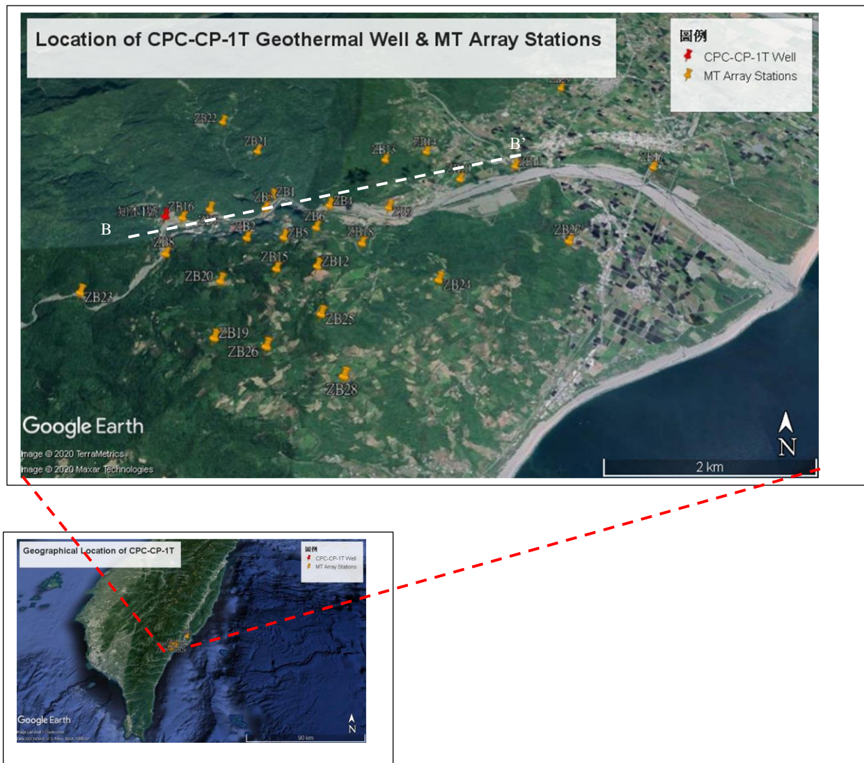
Figure 3 : The figures show the geographical locations of CPC-CP-1T geothermal well and the MT Array Stations. Also shown is the location of B-B' profile.
