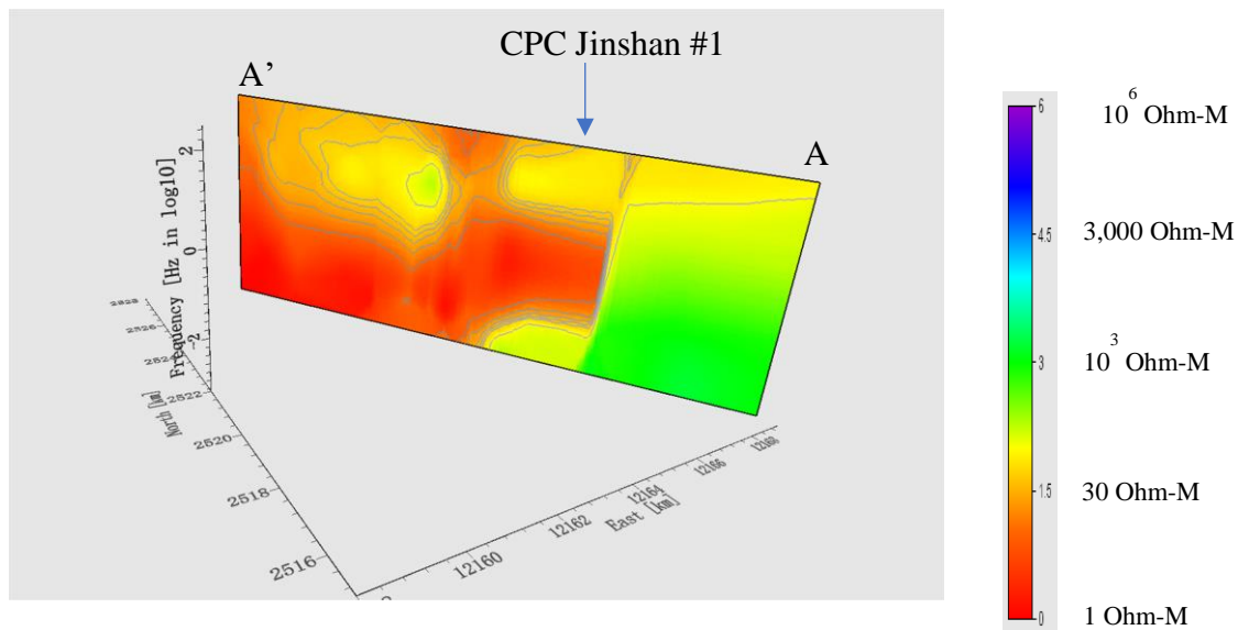
Figure 7 : The apparent resistivity distribution with respect to frequency along profile A-A' interest with CPC Jinshan #1 well.
