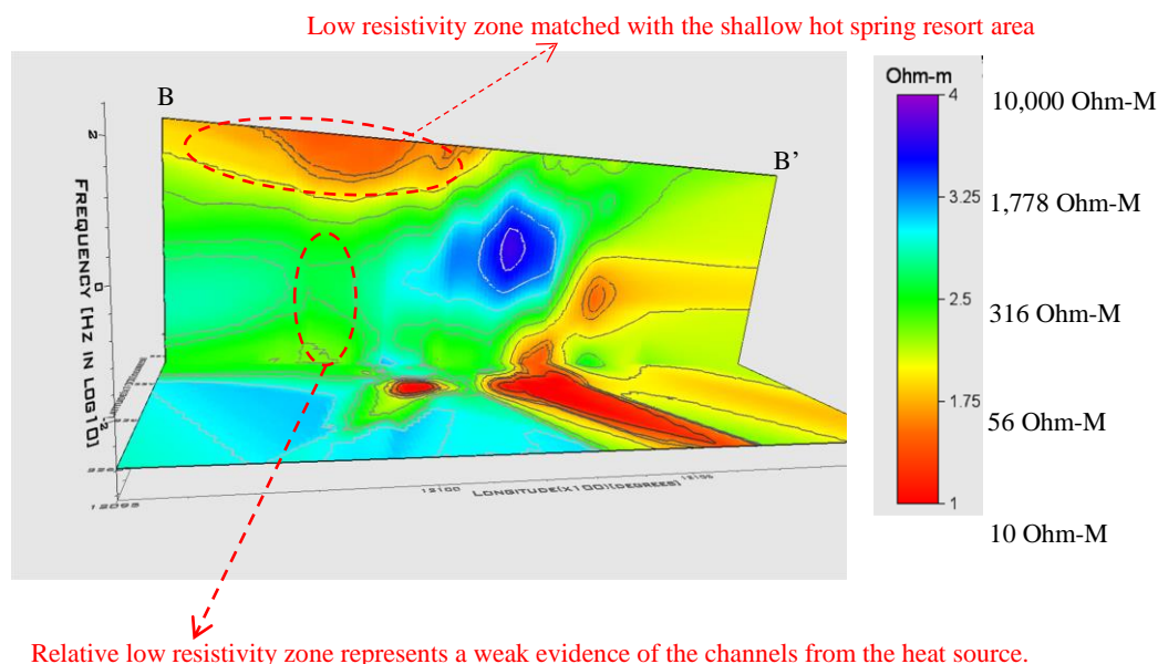
Figure 5 : The effective apparent resistivity distribution with respect to frequency from the MT Array along B-B' profile as shown on Figure 3.
