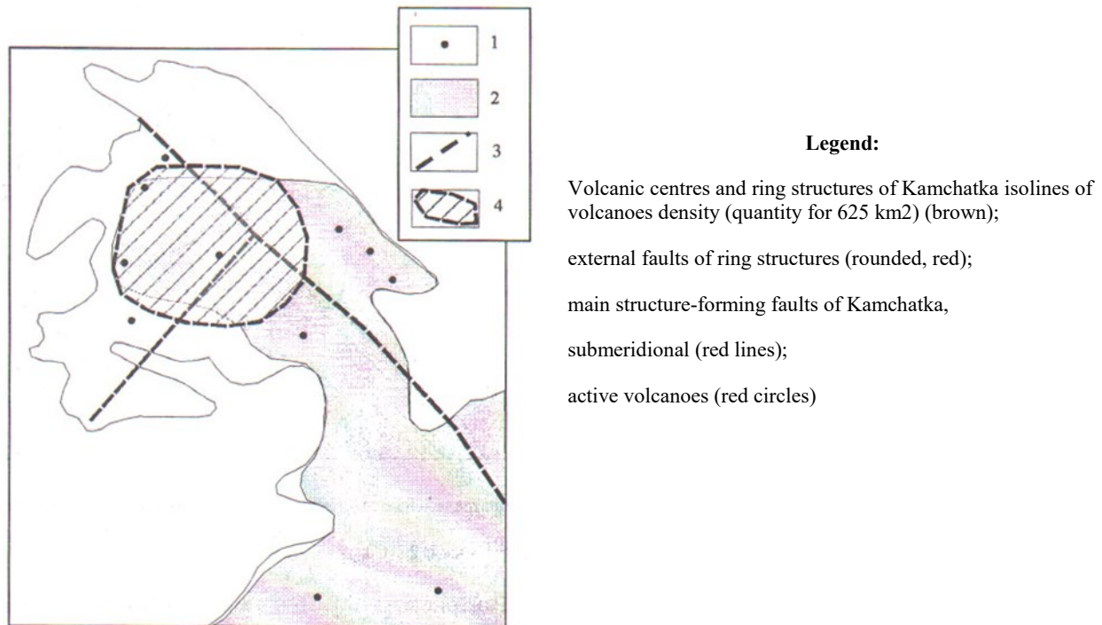
Fig. 7. Tectonic map of the Avacha Bay
