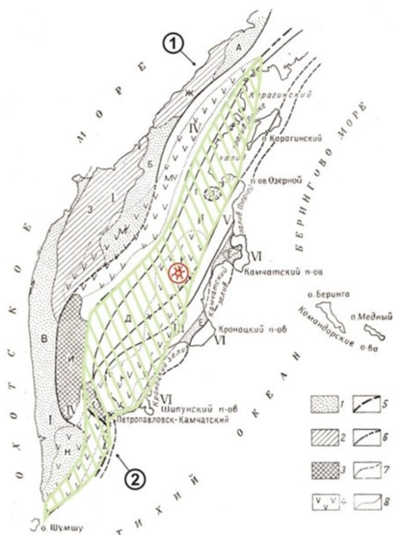
Fig. 8. Predominant structure-forming faults of Kamchatka noted during the studying active volcanoes in dynamic systems of volcano centres by Yu P Masurenkov [1]
