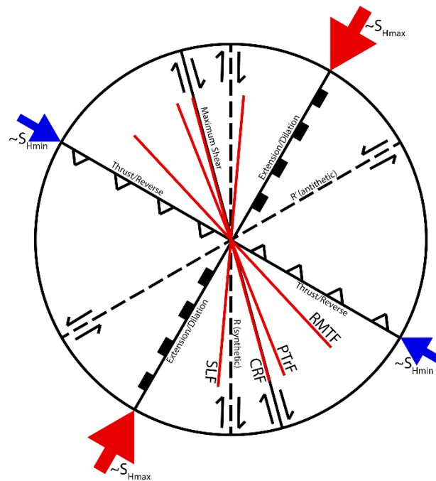
Figure 8. Strain ellipse for approximate S_{Hmax} orientation in southeastern BC (Ristau et al., 2007), and corresponding predicted modes of brittle deformation on faults and fractures. Average orientations of the Rocky Mountain Trench Fault (RMTF), Purcell Trench Fault (PTRF), Columbia River Fault (CRF), and Slocan Lake Fault (SLF), are shown for reference.
