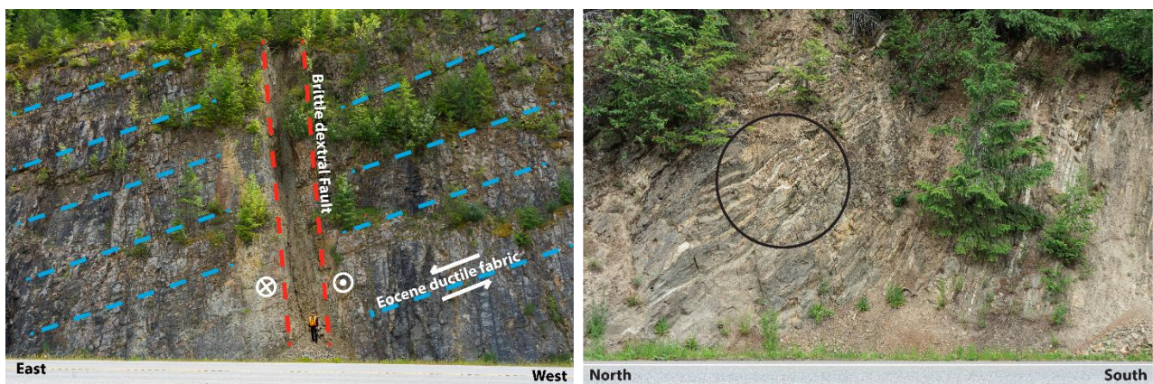
Figure 4. A) A) View south at outcrop on Highway 6 south of New Denver (49.8189 °N, -117.4549 °W). A 2-meter wide subvertical brittle dextral fault oriented 172°/74° cuts across shallowly-east-dipping (008°/31°) ductile fabric of the Slocan Lake Fault/Valkyr Shear Zone. B) View east at outcrop on Highway 6 north of New Denver (50.0555 °N, -117.4323 °W). Small, 20 cm wavelength, south-vergent folds are observed in felsic sills intruded parallel to the S1 cleavage (oriented 278°/51°) of the Slocan Phyllite. Circle is approx. 1.5 m wide.
