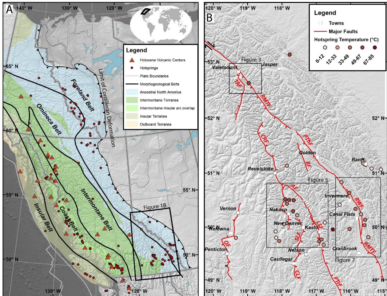
Figure 1. A) Regional geological setting of the Canadian Cordillera. Morphogeological belts are after Gabrielse et al. (1991), and the boundaries of allochthonous and autochthonous superterrains are after Colpron and Nelson (2011). Holocene-active volcanoes (American Geological Institute, 2003) occur predominantly within the Coast Belt. Concentrations of thermal springs occur along the axis of the Coast Belt, in the northern Omineca and Foreland Belts, and in the southern Omineca and Foreland Belts (Woodsworth and Woodsworth, 2014). Note that the latter two clusters do not correspond to regions of active volcanism, but do correspond to significant ( >100 mW/m 2 ) heat flow anomalies (see: Majorowicz and Grasby, 2010). Our study areas are located in the southern Omineca and Foreland Belts. B) Major faults in southeastern British Columbia: AF—Adit Fault; BF—Beaver Fault; CLF—Champion Lakes Fault; CRF—Columbia River Fault; LSF—Lakeshore Fault; OF—Okanagan Fault; PThF—Purcell Thrust Fault; PTRF—Purcell Trench Fault; RMTF—Rocky Mountain Trench Fault; RWF—Redwall Fault.
