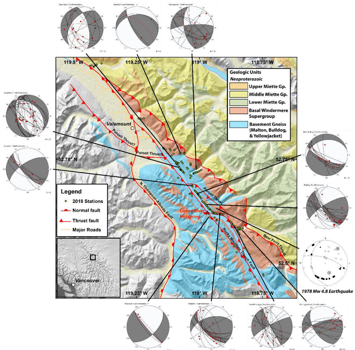
Figure 3. Geology map of Canoe Reach on northern Kinbasket hydroelectric reservoir, south of Valemount, BC after Murphy, (2007). Green dots are sites examined in the field. Lower-hemisphere stereonets show fault plane and slickenline orientations for subsets of stations along Kinbasket Lake. P and T quadrants represent the average kinematics for each subset. The focal mechanism for the 1978 M 4.8 McNaughton Lake earthquake (Rogers et al., 1980) is provided for comparison (lower right).
