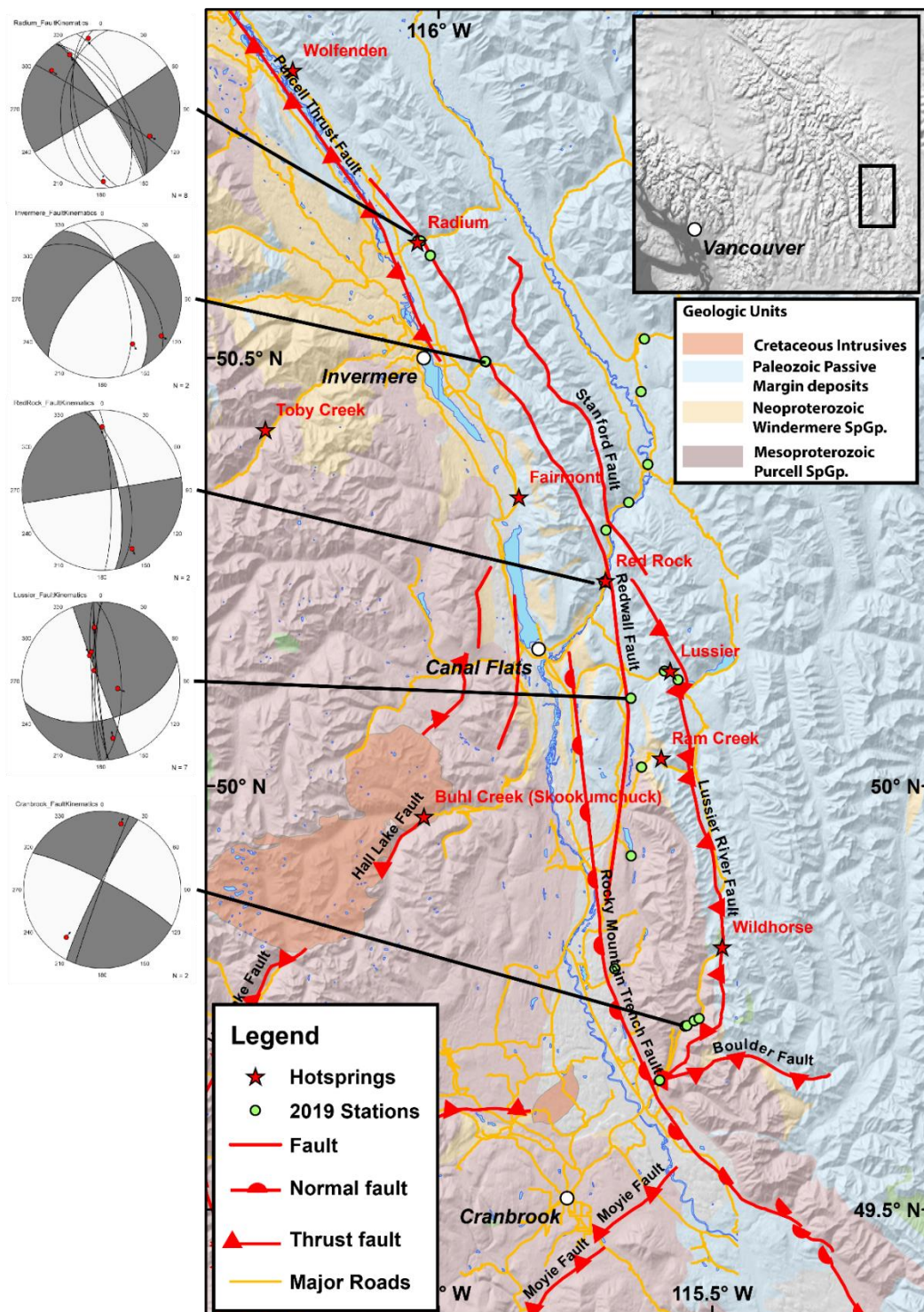
Figure 7. Geology map of the Southern Rocky Mountain Trench from Radium to Cranbrook, after Cui et al. (2017). Lower-hemisphere stereonet plots show fault plane and slickenline orientations for subsets of stations. P and T quadrants represent the average kinematics for each subset. Dextral fault kinematics were observed on the Redwall Fault at several locations.
