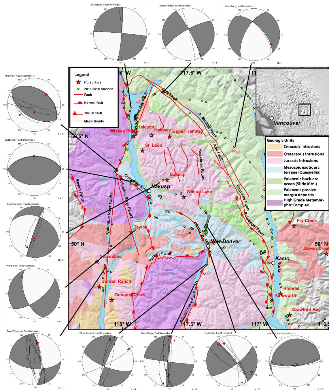
Figure 5. Geology map of the West Kootenay region around Nakusp, BC, after Cui et al., (2017). Lower-hemisphere stereonets show fault plane and slickenline orientations for subsets of stations. P and T quadrants represent the average kinematics for each subset. Dextral kinematics were observed on the Columbia River and Slocan Lake Fault, while reverse kinematics were observed in the transfer zone between Nakusp and New Denver.
