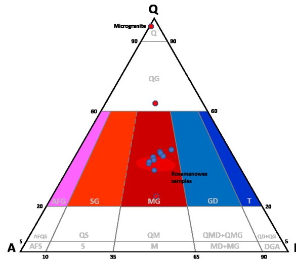
Figure 5. QAP classification of UD-1 granites (coarse cuttings 720-5275 m analysed by QEMSCAN). Almost all samples plot within the monzogranite field and are similar to the granites in the nearby Rosemanowes HDR site (red elliptical field). UD-1 samples in red have anomalous compositions due to cuttings representivity or alteration (microgranite).
