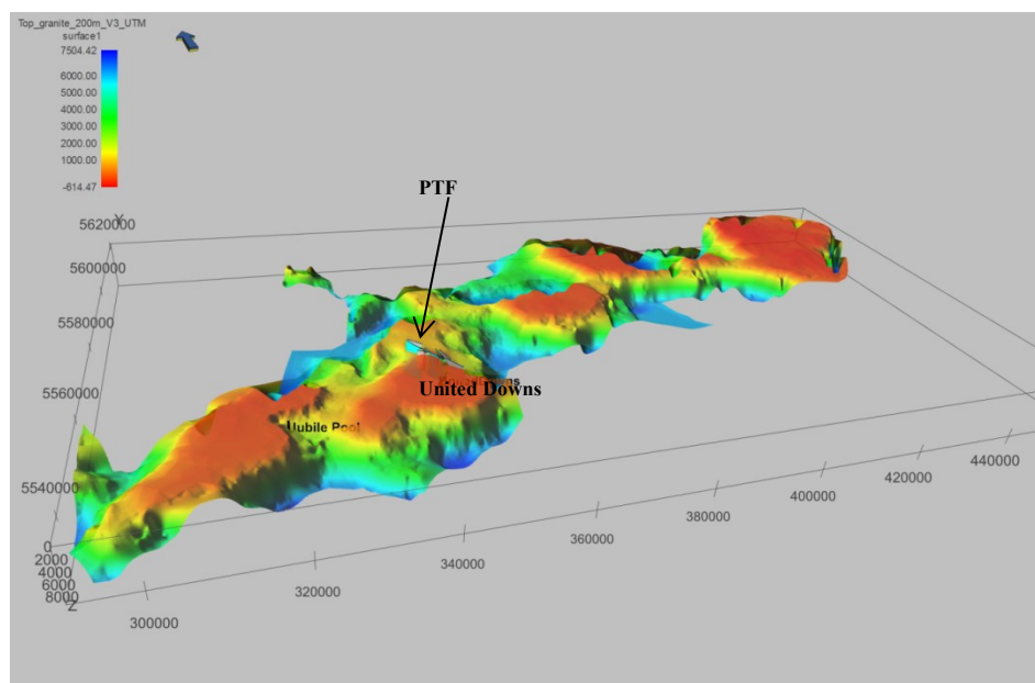
Figure 3: RMS model showing interpreted depth to granite from gravity data interpreted by Willis-Richards and Jackson (1989).
