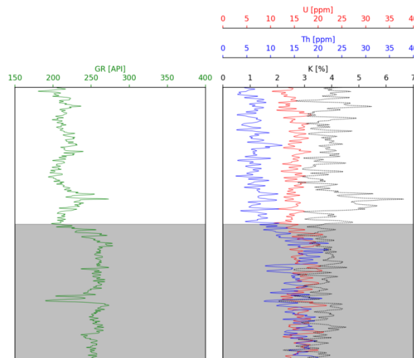
Figure 6: the boundary between two granite types in UD-1 where a sustained increase in Th occurs (shaded white/grey).
