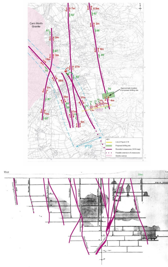
Figure 4a: Map of the PTF structures as seen from surface mapping and mine data. Lateral offsets shown in red, dip directions and magnitudes in green. The PTF envelope is outlined with blue dashes, with the drill pad location shown as a green rectangle. The location of the cross-section shown in Figure 4b is shown in yellow.
