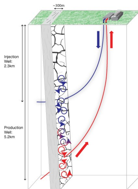
Figure 2: Concept image of the United Downs deep geothermal system.
