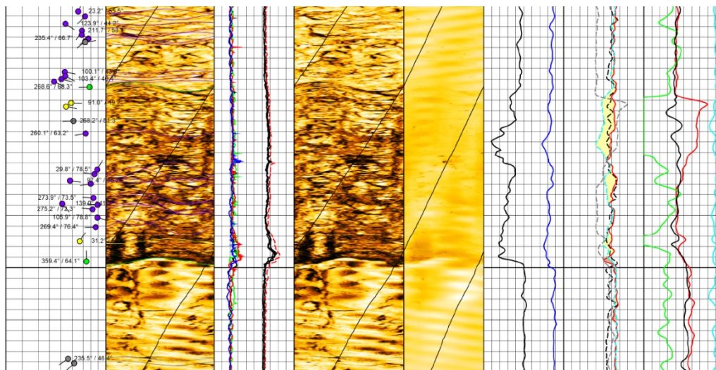
Figure 7. Ultrasonic (UXPL) image log showing a fault zone (~18 m thick) in the granite of UD-1.
