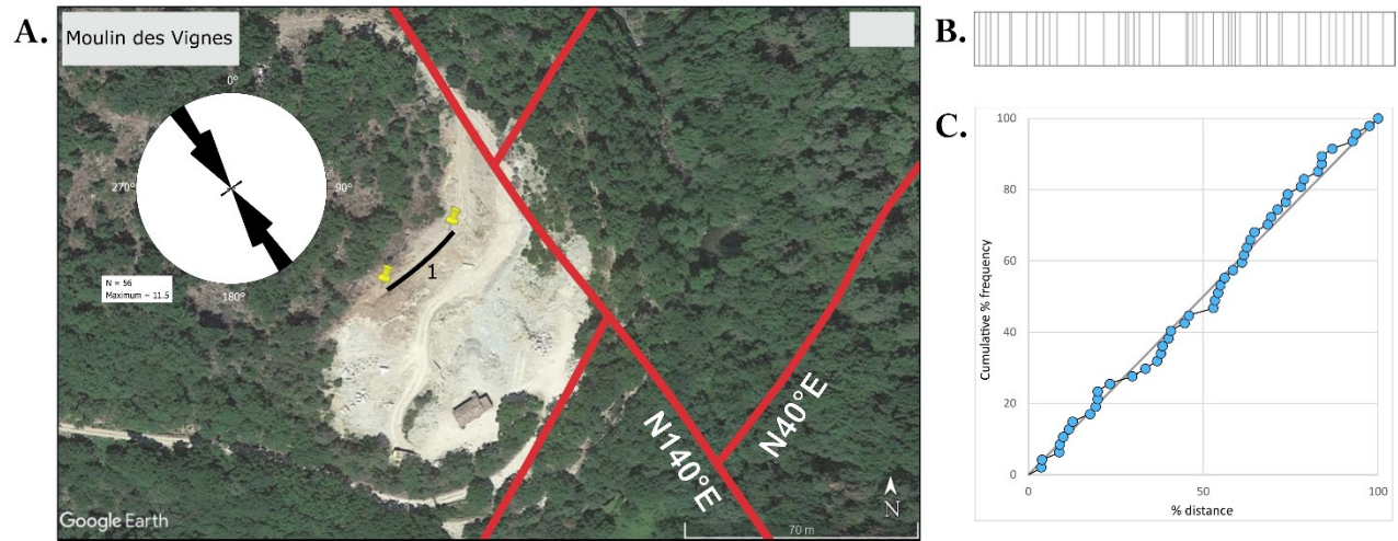
Figure 6: A. Location of the studied profile within the Moulin des Vignes quarry and direction of the fractures measured. Rose diagram of strike direction with 10^\circ classes. Red lines represents the major faults that are indicated on the geological map of Privas at 1:50,000 scale (Ledru et al. , 2014). B. Spatial distribution of fractures on the line represented as stick plots. C. Cumulative plot of % frequency against % distance for the Moulin des Vignes profile. Blue circles show cumulative % frequency and diagonal line represents a uniform distribution.
