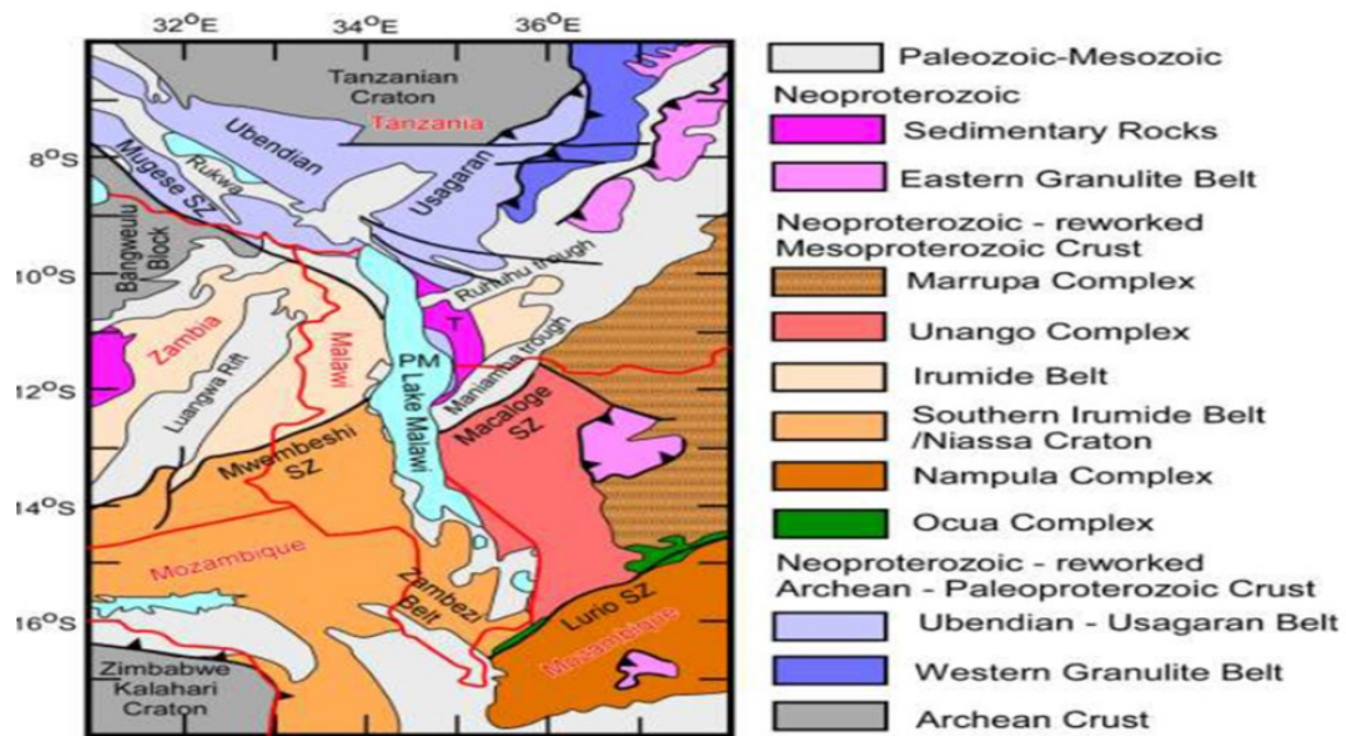
Figure 1: Tectonic map showing the exposures of the Precambrian and Paleozoic-Mesozoic units around the Malawi Rift. (Njinju 2016)
