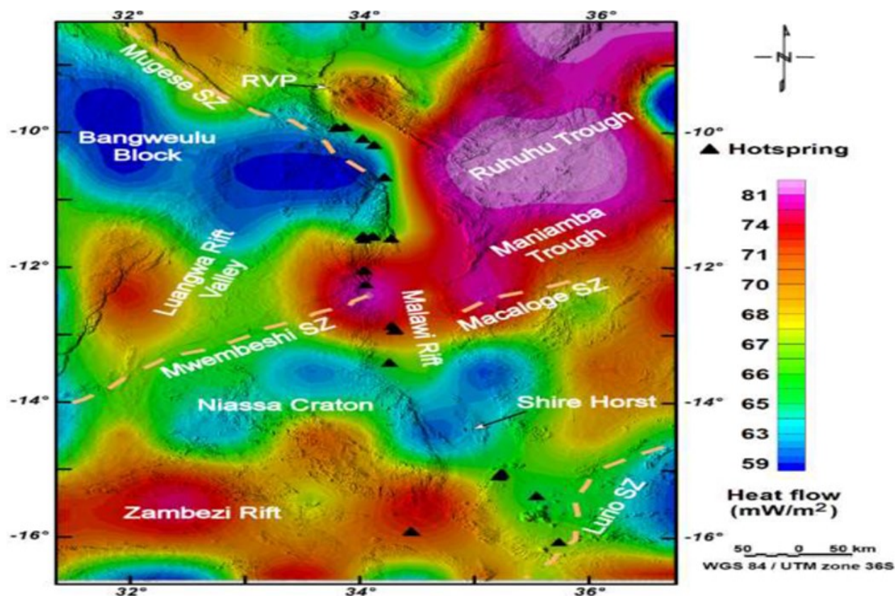
Figure 4: Heat flow and hot spring location map. (Njinju,2016)
