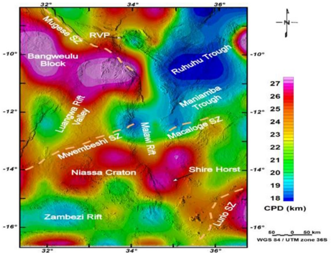
Figure 3: Curie Point Depth Map of Malawi and surrounding areas. (Njinju, 2016)
