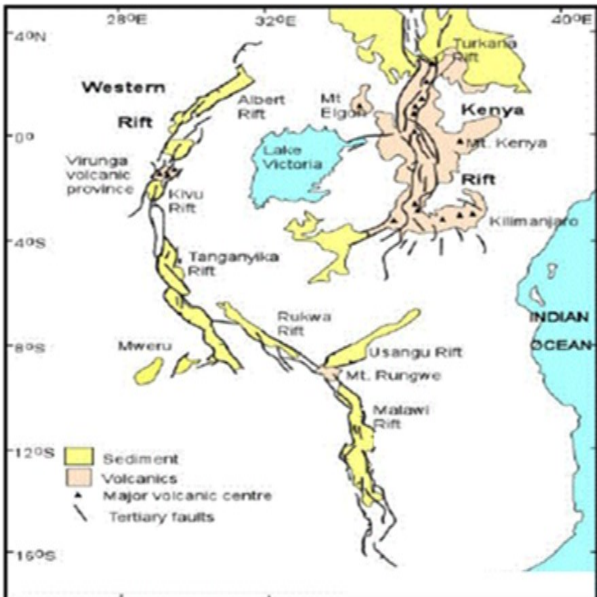
Figure 2: Map showing the Western Branch of the East African Rift Valley System (Omenda, 2010)
