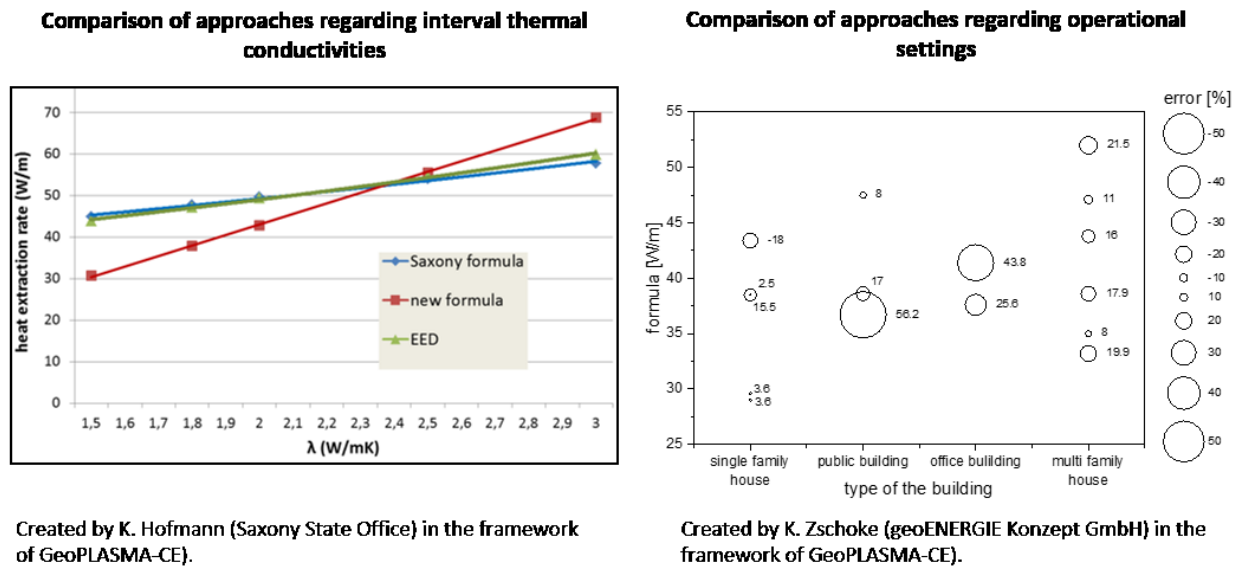
Figure 4: Comparison of the infinite line source method with an empiric formula and the standard software EED for estimating the heat transfer rate of a borehole heat exchanger.
