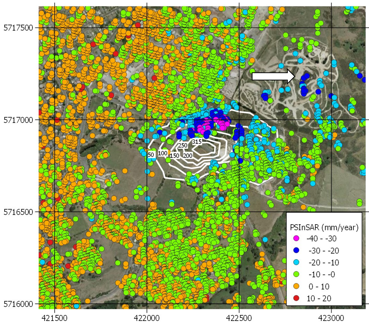
Figure 8 PSInSAR ground motion vertical velocities (2018-2019) overlaid upon Contact levelling survey contours (2015-2016). Note: Levelling contours (white box labels, units of mm/year) show same subsidence at the same location to PSInSAR. Large white arrow points to subsidence near the motocross park.
