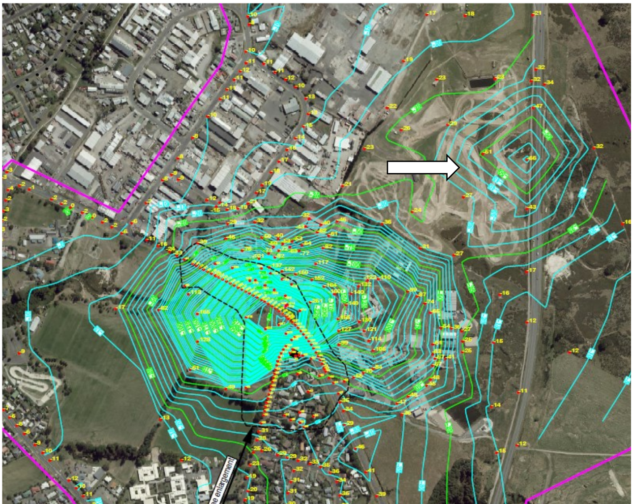
Figure 4 Crown Rd subsidence bowl contours from ground-based levelling survey data. Survey commissioned by Contact Energy and conducted 2015-2016. Large white arrow points to possible additional area of more subtle subsidence centred near the motocross park
