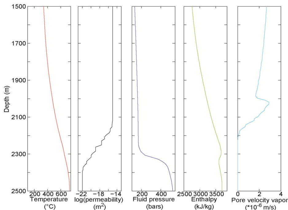
Figure 3. Changes in temperature, permeability, fluid pressure, enthalpy and pore velocity vapor in the zone of superheated steam above the intrusion, along the black line shown in Figure 2.
