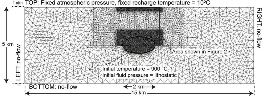
Figure 1. Model set-up, finite element discretization and boundary conditions.
