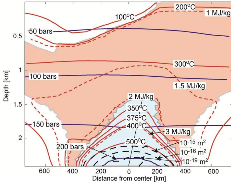
Figure 2. Snapshot showing the state of the system after 2500 years of evolution. Fluid pressure contours are shown by blue lines, temperature contours by red lines, enthalpy contours in dashed red lines, and permeability contours in dashed black lines. The red region represents zones of boiling, while the blue region represents a zone of a single-phase fluid with vapor-like density. White represents single-phase fluid with a liquid-like density.
