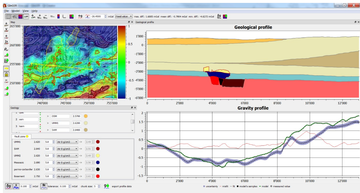
Figure 4: Print screen of GInGER made with Quaternary structures, Permo-Carboniferous graben and fractured zone added. On gravity profile, blue line: measured gravity with uncertainty, green line: model's gravity effect, red line: misfit.
