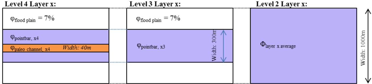
Figure 10: Schematic top view of reservoir model layers of level 4 to 2. The floodplain fines are white, point bar sandstone is purple and paleo-channel orange. On the right layer x of level 2 with only sandstone facies.
