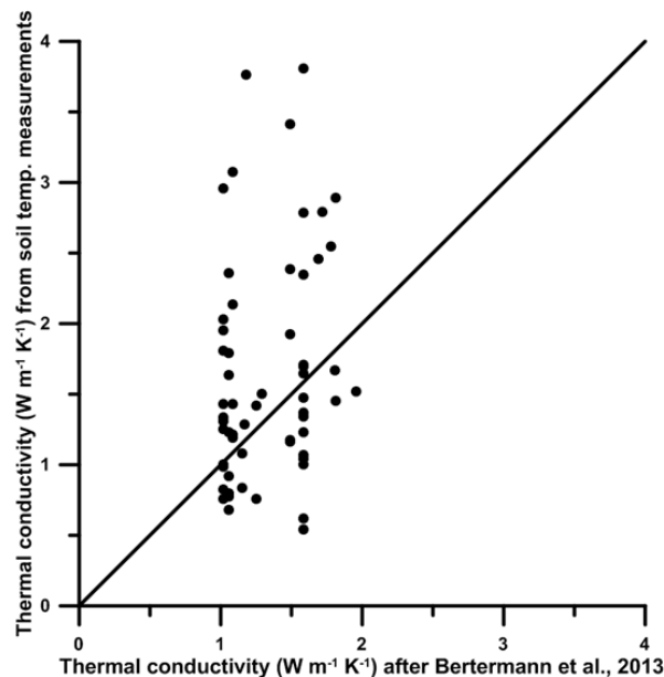
Figure 6: Plot of estimated thermal conductivities derived from the soil temperature measurements against those derived by the methodology of Bertermann et al. (2013). The solid line is the line of correlation between the two data sets.
