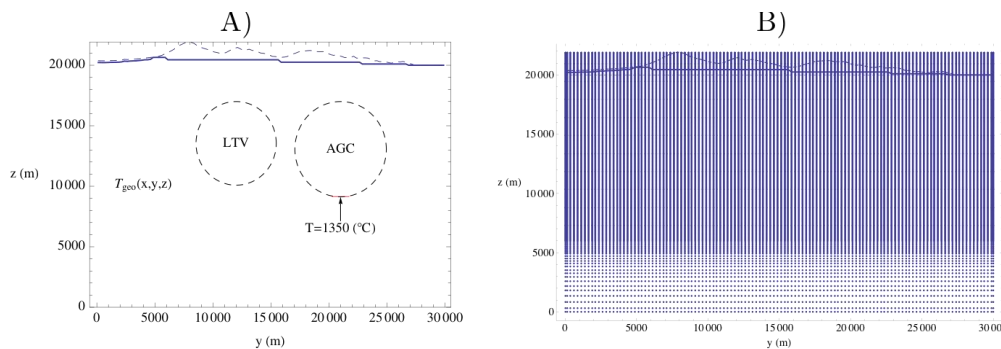
Figure 5: A) Cross section ( x=10,000 m; Fig. 2) illustrating the initial condition of the problem. The top boundary (solid curve) has a specified temperature ( 25^\circ\text{C} ). Dashed circles define the region where the chambers will be emplaced with initial temperature of 1350^\circ\text{C} . B) Density distribution of control volumes for the numerical model.
