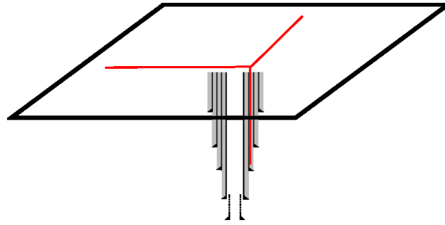
Figure 1: Conceptual design of the fiber-optic installation within the IMAGE project (not to scale). The cable (red) will be installed down to a depth of 1200 m. Some additional cable length shall be deployed at the surface to create a three dimensional sensor array.
