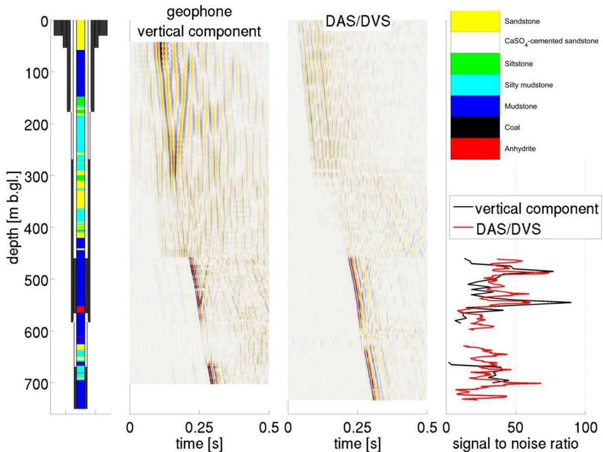
Figure 2: (left to right) Well completion of well Ktzi 202, vertical component of conventional geophone, processed data from DAS/DVS survey, well lithology and signal-to-noise ratio comparison for the depth interval 450-700 m. The optical fiber is installed behind the production casing. Cemented intervals are indicated by gray section in the well diagram.
