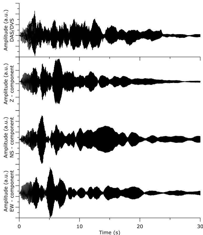
Figure 3: Comparison of measured signal from the optical fiber buried in a 50 cm deep trench (top) below a three component geophone (three traces at the bottom).
