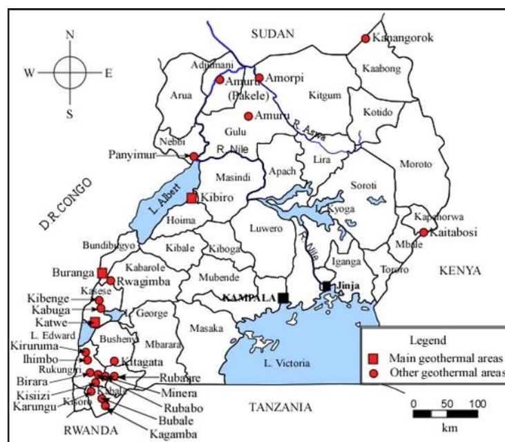
Figure 2. The geothermal areas of Uganda
