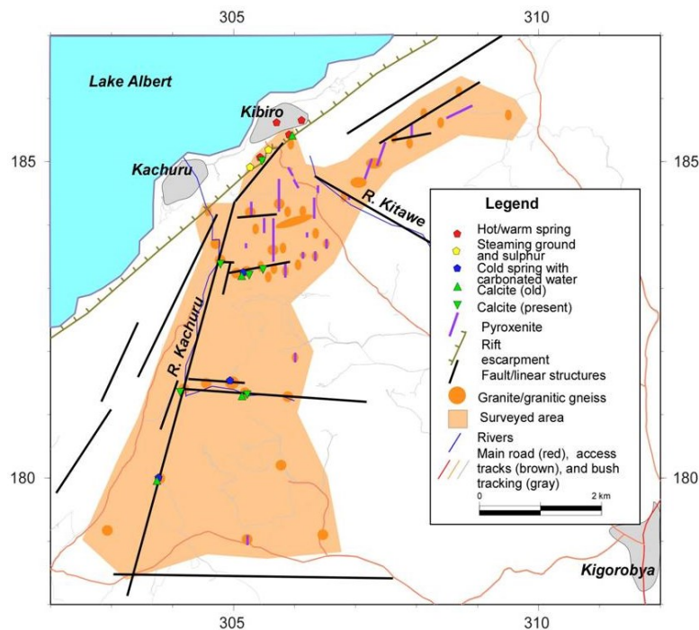
Figure 3. Geologic map of the Kibiro area.
