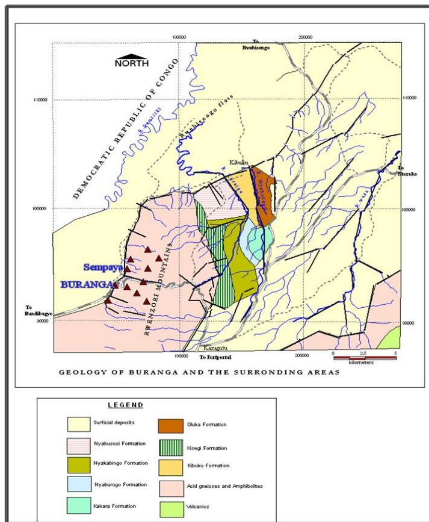
Figure 12: Geologic map of Buranga showing location of hot springs.
