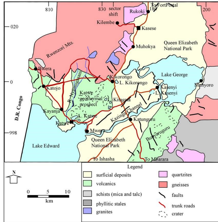
Figure 8. Geologic map of Katwe area and its surroundings.
