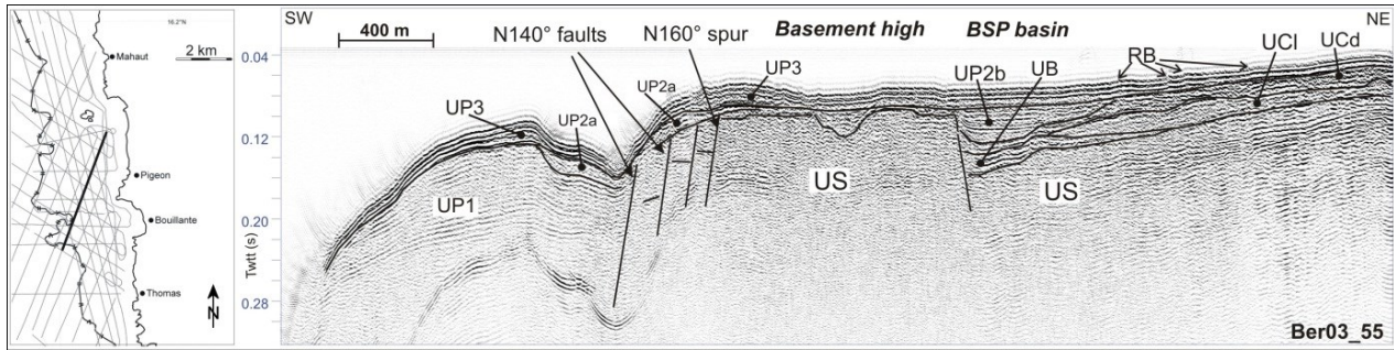
Figure 3: A Geoberyx03 VHR seismic profile (Thinon et al., 2010) showing the sedimentary cover (UP, UC, RB, UB), the acoustic basement (US), and the major faults. RB: surficial formation. Various seismic units are noted (names starting by U). Location of the marine seismic section on the left hand side (West Guadeloupe offshore).
