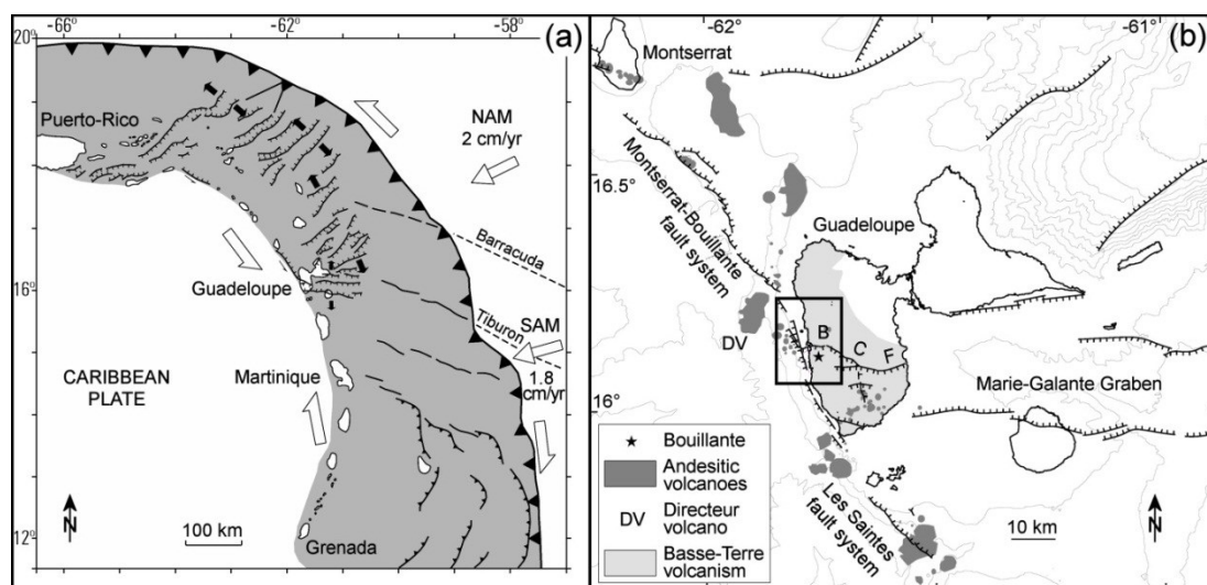
Figure 1: (a) Geodynamic context of the West Indies (modified from Feuillet et al., 2002). NAM: North American plate. SAM: South American plate. (b) Regional structural setting of the Guadeloupe Island (modified from Thinon et al., 2010). Thick square: location of the 3D fault model. BCF: Bouillante-Capesterre fault system.
