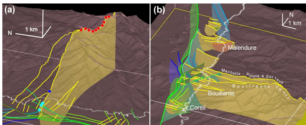
Figure 4: Two views of the fault model achieved for the Bouillante geothermal province (see Fig. 3a for location). The coastline (white crosses) separates onshore and offshore domains. a. The Bouillante fault (yellow surface) is constructed from onshore field observation (dark blue point), onshore interpretation (red points) and offshore seismic profiles interpretation (light blue points). View from WSW. b. The final 3D interpretation reveals three main families of faults (yellow, green, and blue). View from SSE.
