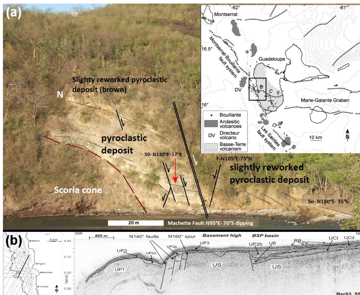
Figure 3: Example of the onshore and offshore knowledge in the Bouillante geothermal province. a. Picture of the Anse Machette inland outcrop at the north end of the Bouillante bay (Bouchot et al., 2010); view from W, see box in b. for location. Box: Regional structural setting of the Guadeloupe Island (modified from Thinon et al., 2010). Thick square: location of the 3D fault model. BCF: Bouillante-Capesterre fault system. b. A Geoberryx03 very high resolution marine seismic profile opposite to the Bouillante bay; see box on the left hand side (Thinon et al., 2010).
