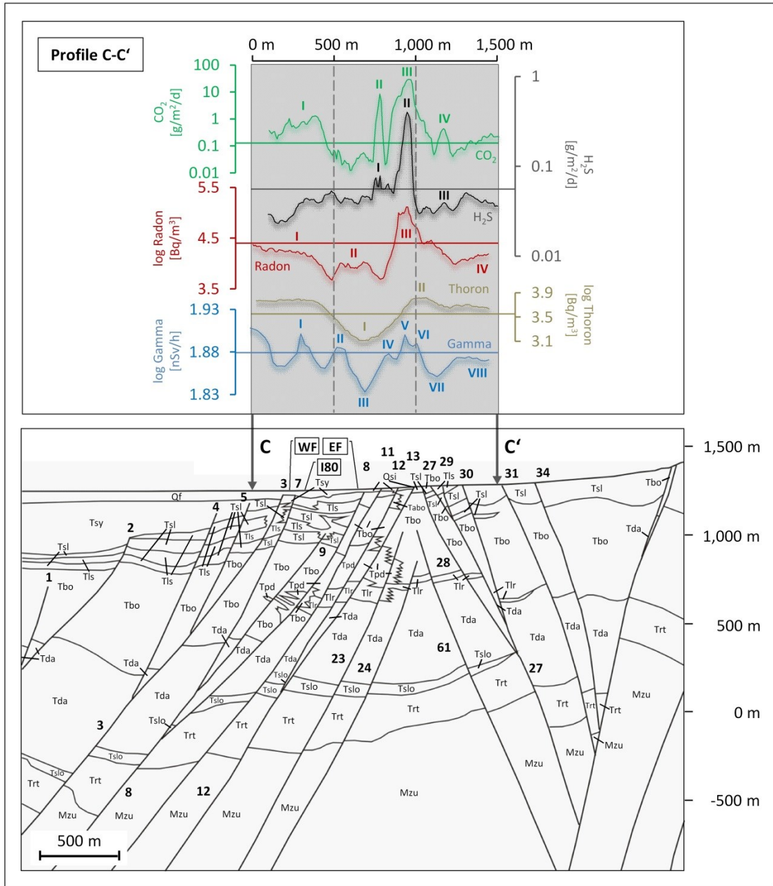
Figure 7: The diagram illustrates the variation of five monitored parameters ( \text{CO}_2 , \text{H}_2\text{S} , ^{222}\text{Rn} , ^{220}\text{Rn} , gamma radiation) along cross section C-C' (geological cross section from Faults, unpublished data, 2011). Horizontal reference lines: \text{CO}_2 = 0.13 \text{ g/m}^2/\text{d} (detection limit); \text{H}_2\text{S} = 0.057 \text{ g/m}^2/\text{d} (detection limit); ^{222}\text{Rn} = \log 4.41 (mean of all data); ^{220}\text{Rn} = \log 3.56 (mean of population PIII); gamma radiation = \log 1.88 (mean of all data). Color-coded Roman numerals along the data curves indicate anomalies and interpretation for each numeral can be found in the text. Arabic numerals are used for fault labeling. WF: Western frontage road; I80: Interstate I80; EF: Eastern frontage road.
