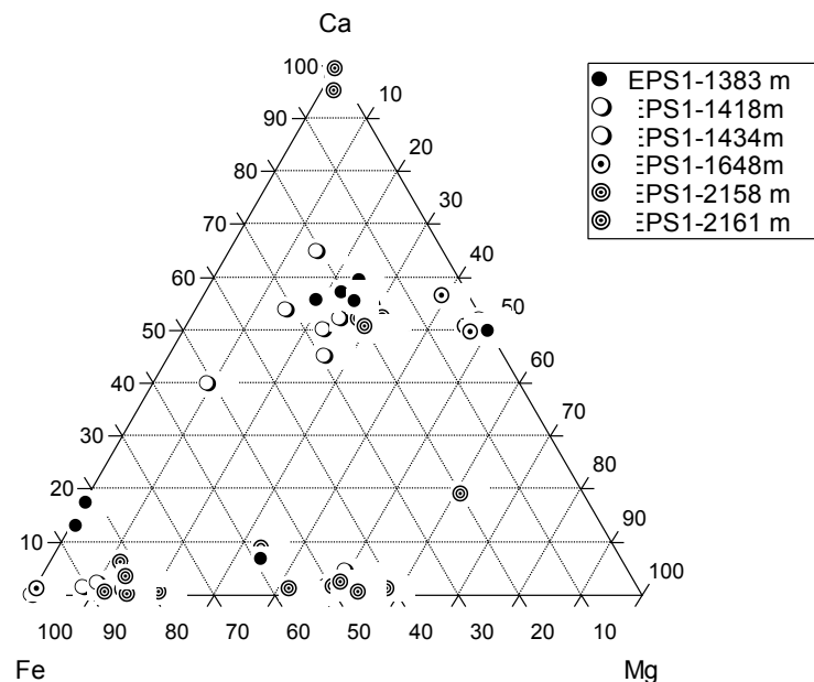
Figure 6 - Ca-Fe-Mg triangular diagram showing the chemical compositions of carbonates (calcite, dolomite, ankerite, siderite) filling fractures crosscutting granite (EPS1-1418 m, 1434 m, 1648 m, 2158 m and 2161 m) and cementing sandstones (EPS1-1383 m) close to the granite interface. Analyses were performed using electron microprobe.
