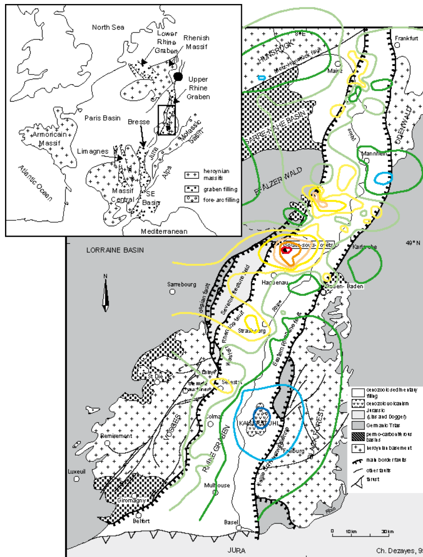
Figure 1: Location and simplified geology of the Upper Rhine Graben. Colored curves indicate isotherm at 1500m to 130°C (red) to 50°C (blue) (data from GGA).
