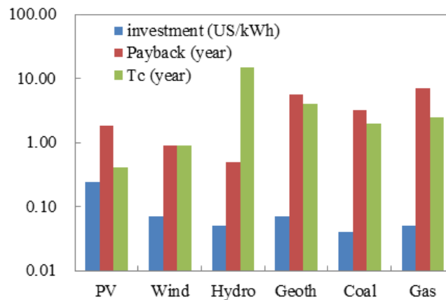
Figure 7: Comparison of cost, initial investment, payback time, and construction period.
