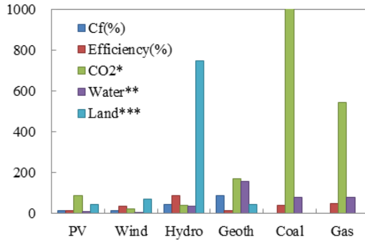
Figure 8: capacity factor, efficiency, and environmental impacts.
