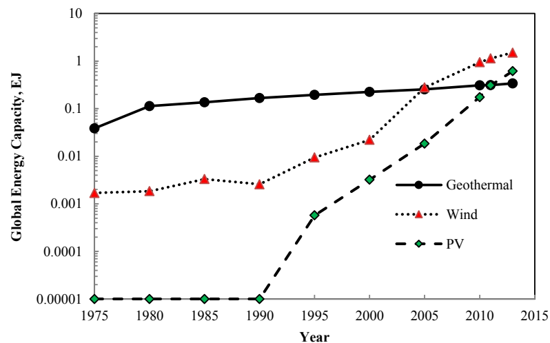
Figure 9: Comparison of generated energy for individual energy type.
