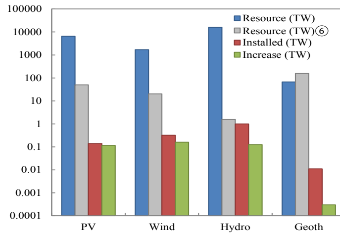
Figure 4: Resources, installed capacity and the increase in the last three years.
