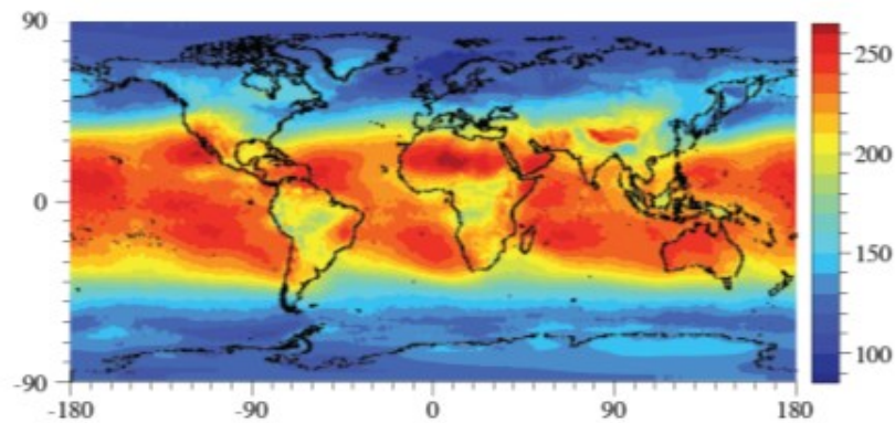
Figure 2: Modeled world Surface radiation ( \text{W/m}^2 ) (global average: 193; land: 185).
