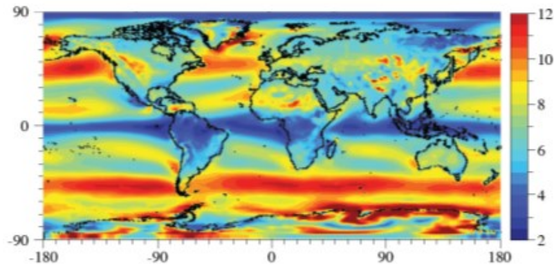
Figure 1: Modeled world Wind speeds at 100 meter.
