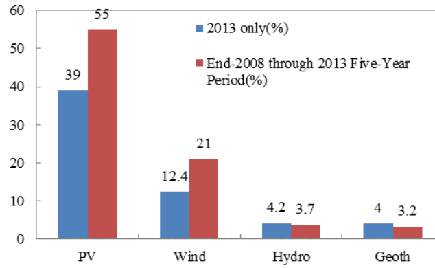
Figure 6: Average annual growth rates of renewable energy capacity, 2008–2013 (Source: REN 21, 2014).
