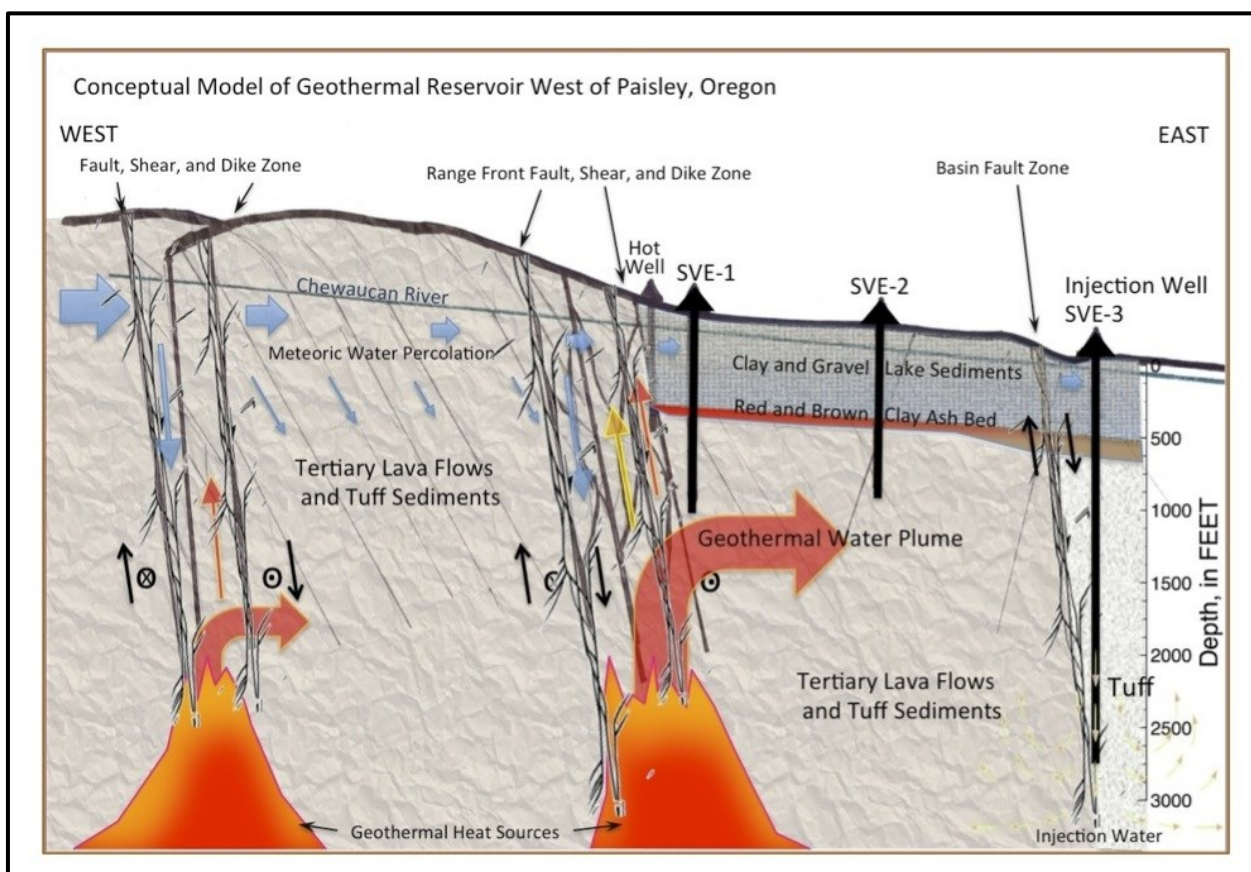
FIGURE 6. Conceptual model of the geothermal reservoir west of Paisley.
