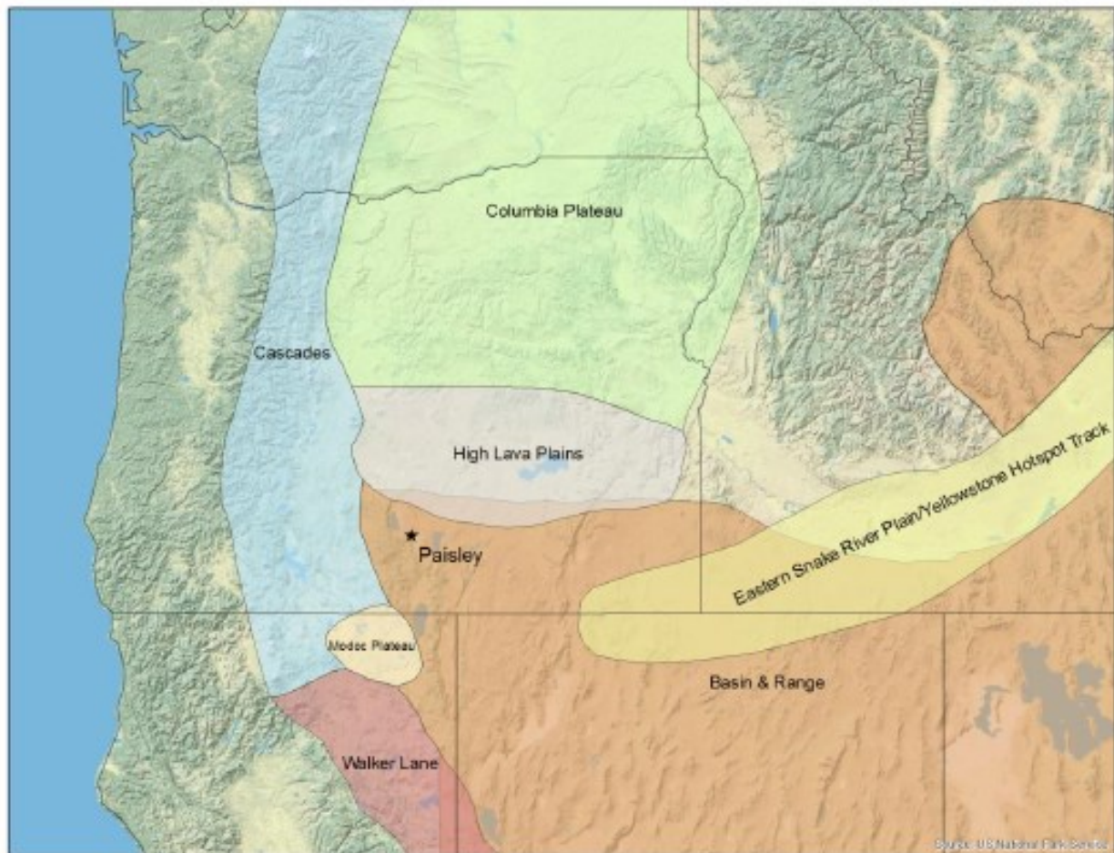
FIGURE 3. Physiographic Provinces
