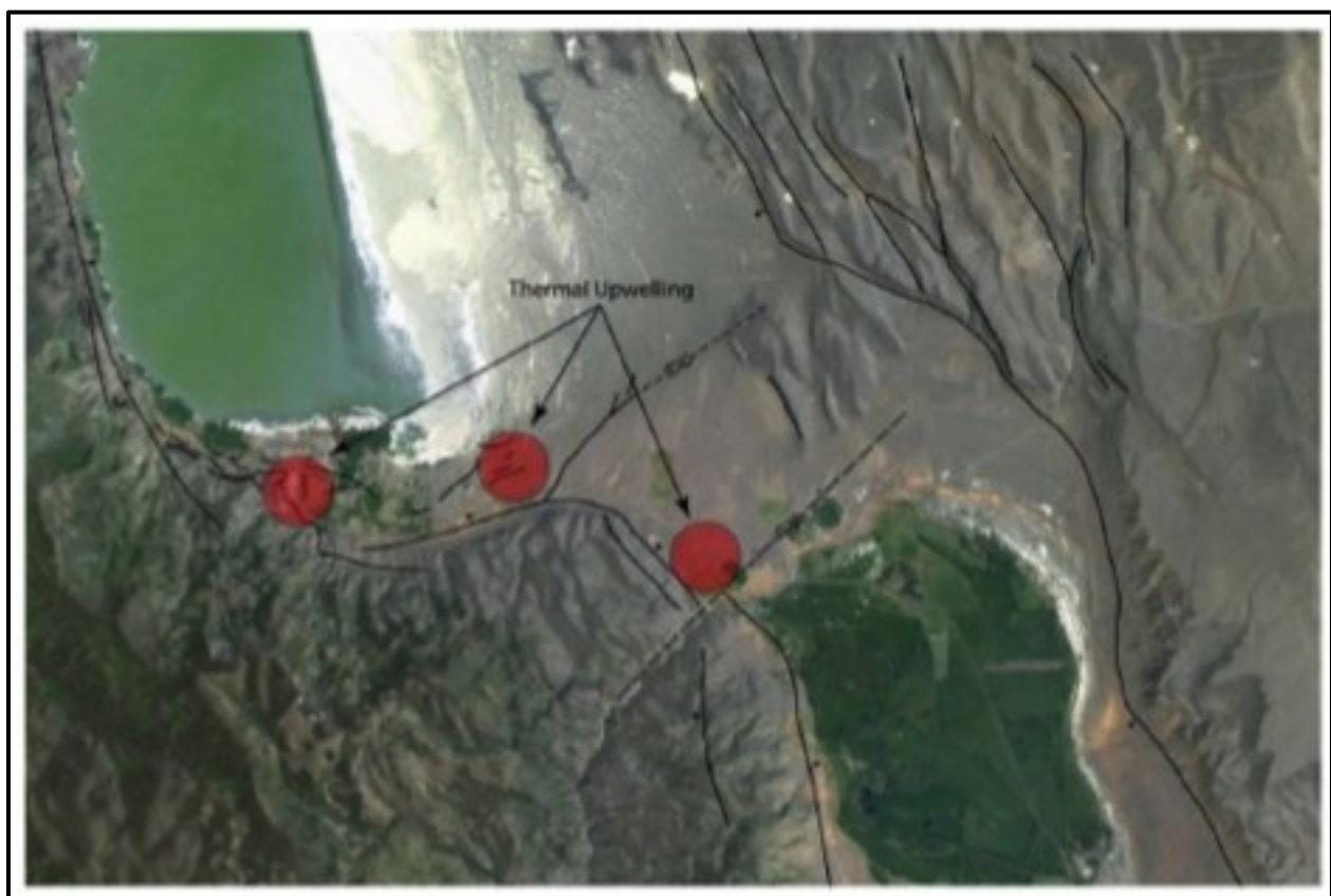
Figure 4. Map of the Paisley Transfer zone. Red circles indicate areas of thermal water upwelling.
