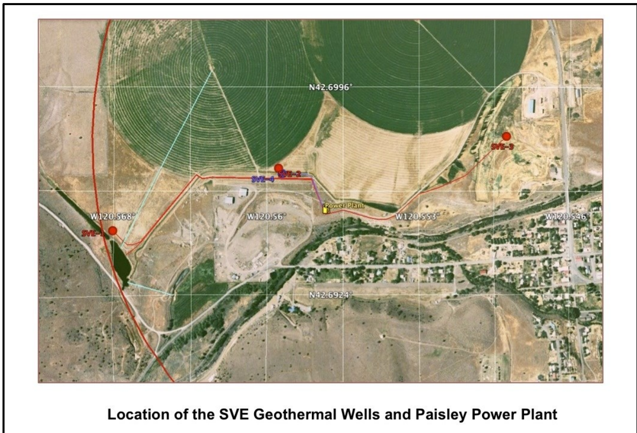
FIGURE 7. Vertical image showing location of Paisley geothermal wells, power plant, and pipelines.
