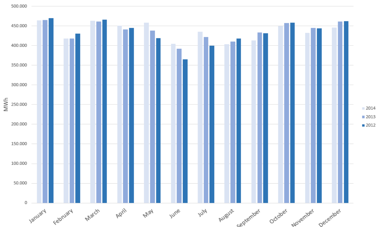
Figure 6: Electricity generation by geothermal power plants per month for the past three years.
