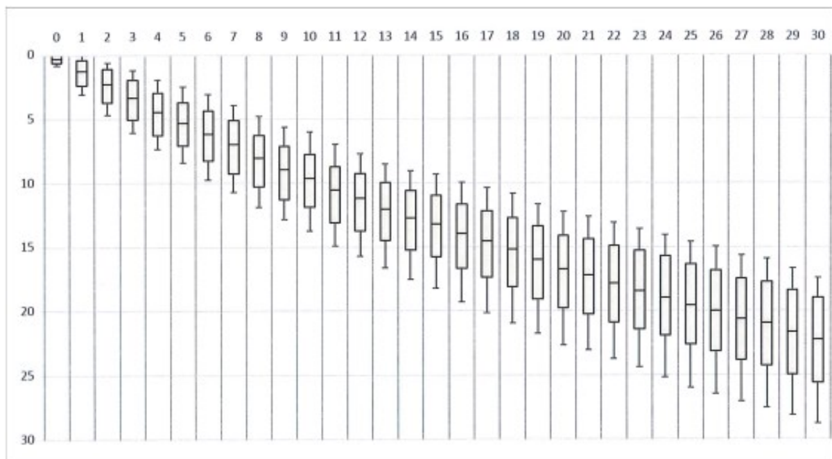
Figure 11: Limitations of drawdown to ensure long-term utilisation of the resource. The vertical scale shows pressure drawdown from natural state in bars. The horizontal scale is in years of operation with an uncertainty margin (Orkustofnun, 2014).
