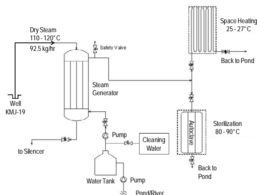
Figure 3: Schematic Diagram of Mushroom Cultivation by Utilizing Steam from Small Production Well
