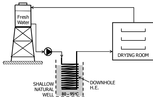
Figure 7: Schematic Diagram of Copra Drying by Utilizing Shallow Natural Well
