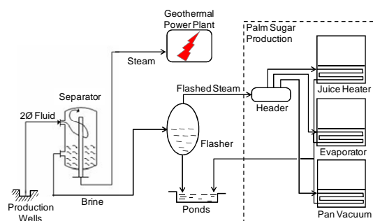
Figure 6: Schematic Diagram of Palm Sugar Production by Utilizing Brine
