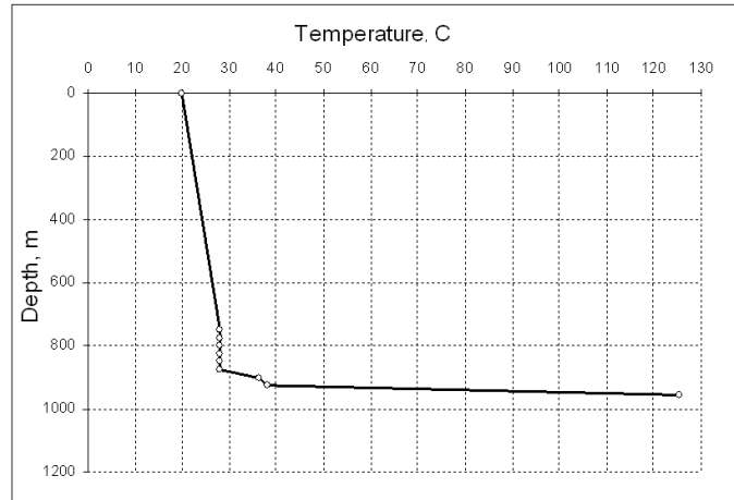
Figure 3: Water loss test conducted in AS-2 well.
