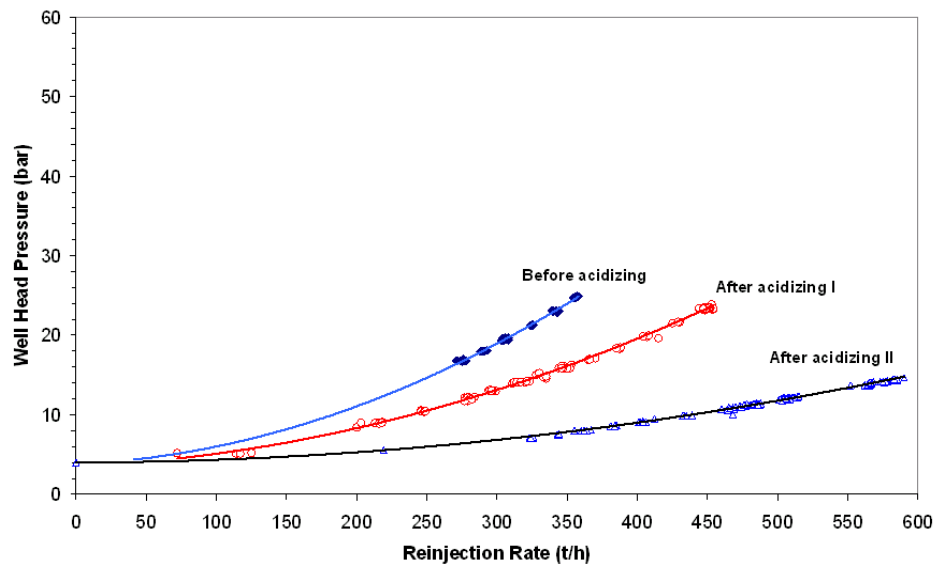
Figure 9: Reinjection history of AS-2 well in 2008-2009 period.
