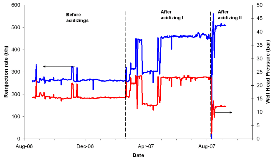
Figure 8. Reinjection history of AS-2 well in 2006-2007 period.
