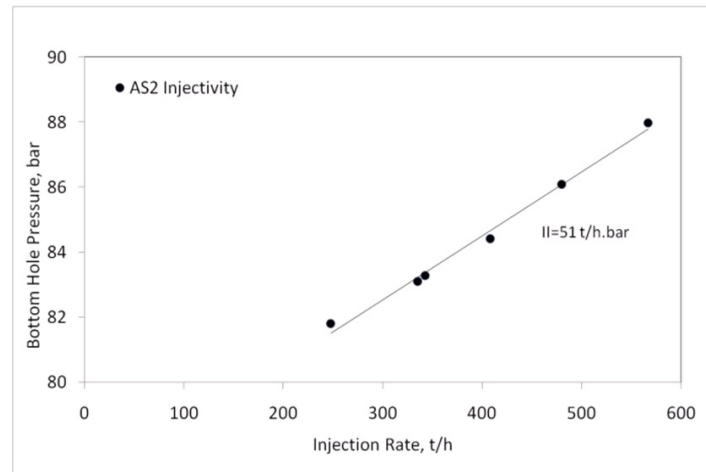
Figure 6: Results of injectivity test in AS-2 well.
