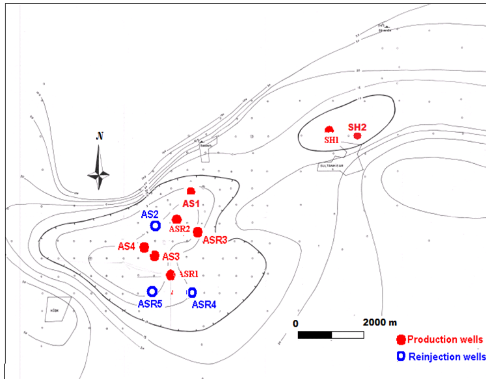
Figure 2: Location of production and reinjection wells.
