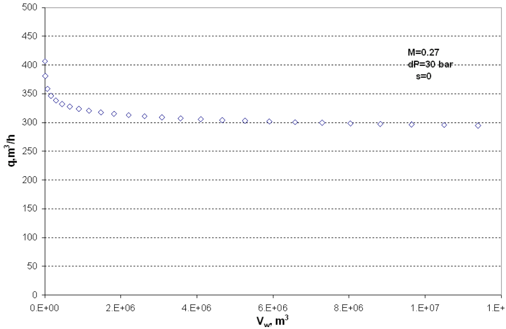
Figure 12: Injection rate vs. injected volume for line-drive solution (Serpén and Aksoy, 2005).
