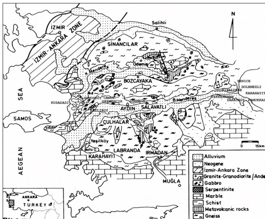
Figure 1: Location and geological map of Büyük Menderes Massif (Serpen et al., 2003).
