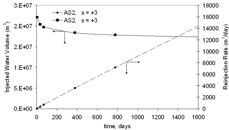
Figure 7: Change of Injection rates and injected volume over time for AS-2 well.
