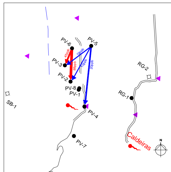
Figure 6: Tracer return pattern at Pico Vermelho
