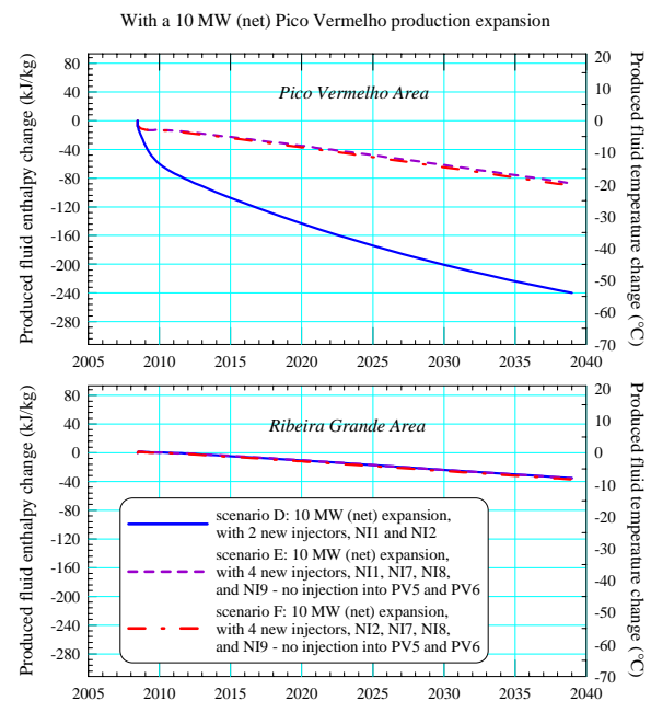
Figure 12: Production enthalpy forecast, scenarios D, E, and F
