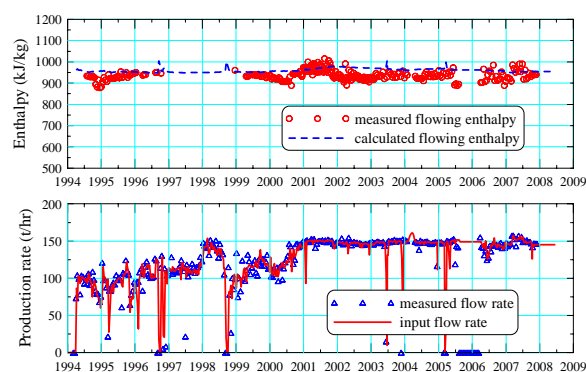
Figure 4: Production parameters matching, well CL1
