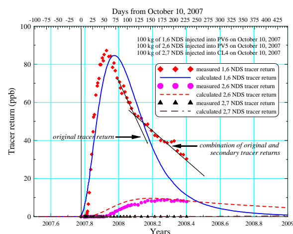
Figure 7: Tracer return matching, well PV2
