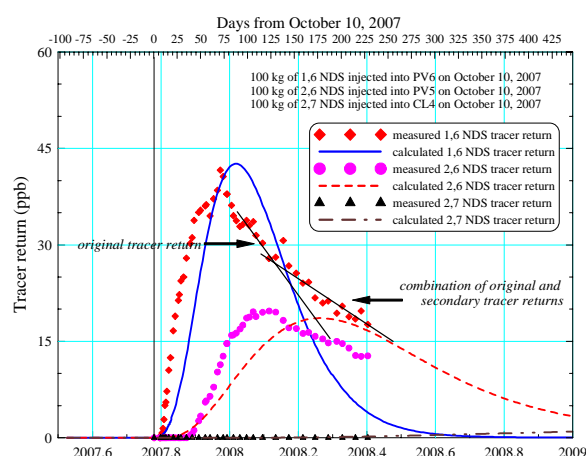
Figure 9: Tracer return matching, well PV4
