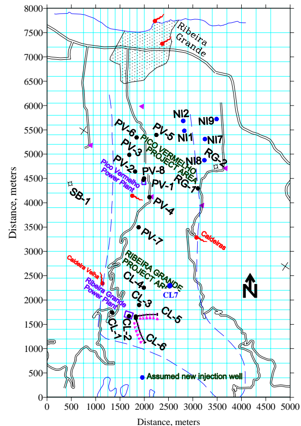
Figure 10: Well locations used in the forecasts
