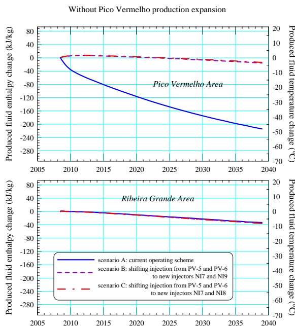
Figure 11: Production enthalpy forecast, scenarios A, B, and C
