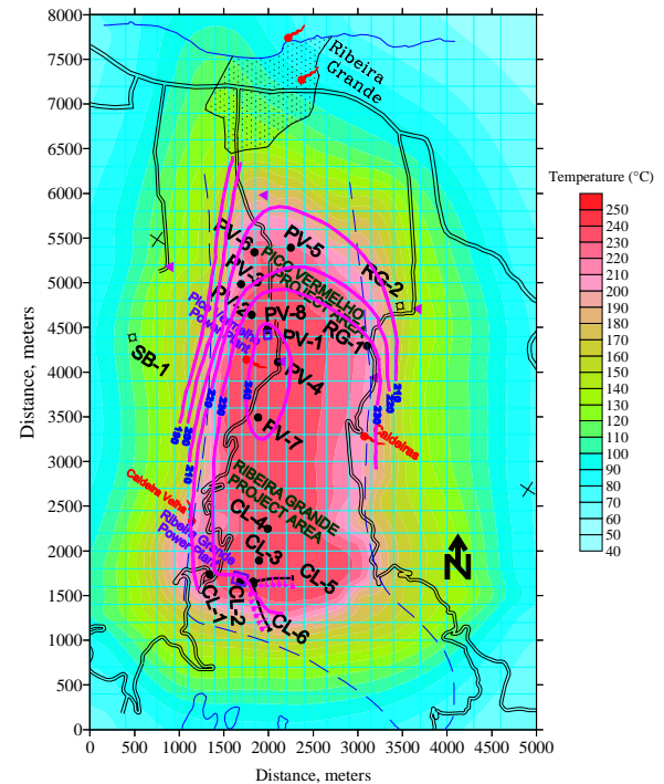
Figure 3: Subsurface temperature matching, layer 3, at -300 meters, msl.
