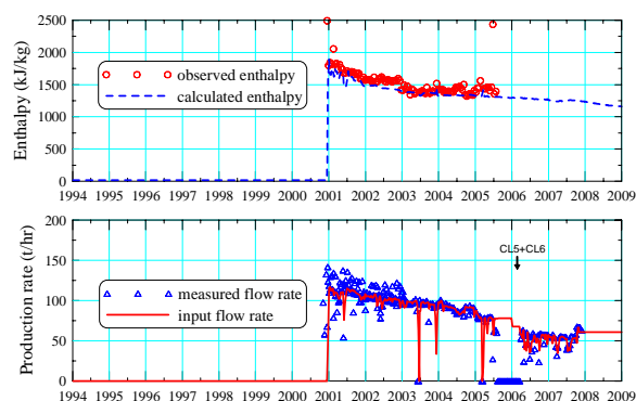
Figure 5: Production parameters matching, well CL5
