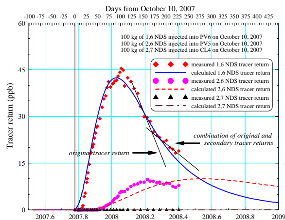
Figure 8: Tracer return matching, well PV3
