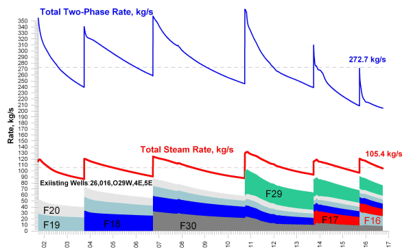
Figure 5: Forecasting modeling (scenario EX3A) of total two-phase, total steam production of wells (existing wells 016, 26, E4, 029W, E5 and additional F-wells) at Dachny site, Mutnovsky geothermal field
