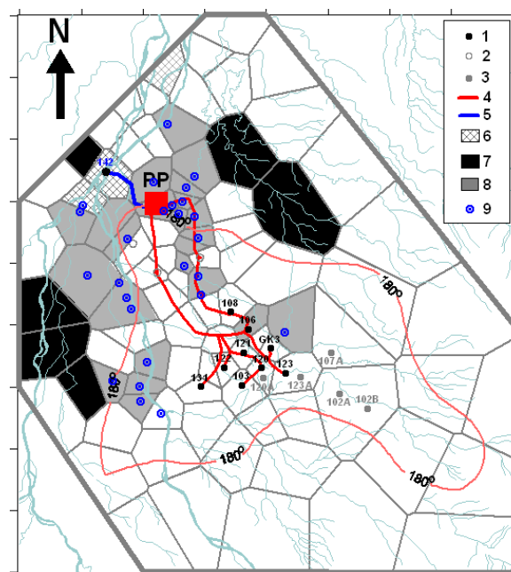
Figure 1: Top view of the numerical grid used to model the Pauzhetsky geothermal field. 180°C isotherm corresponds to the initial temperature at -250 m asl. Well 142: injection well; PP: Power plant. Legend: 1- existing production wells, 2- old production wells, 3- additionally needed wells, 4- steam transmission lines, 5- separate water pipeline, 6- hot spring, areas, 7 - low permeability domains, 8 - infiltration areas, 9 - potential infiltrators - abandoned or monitoring wells inside of the infiltration areas. Grid size 500 m
