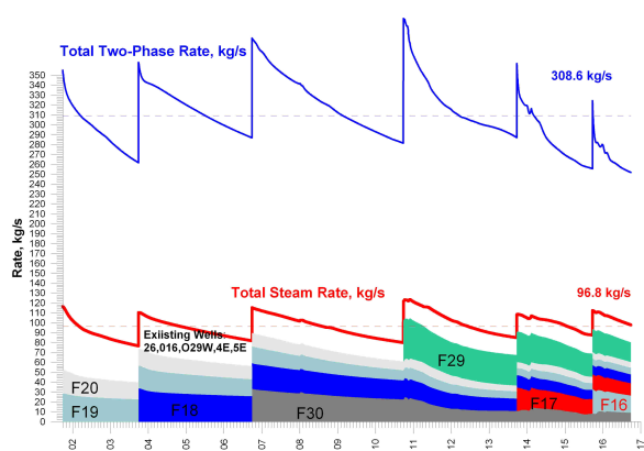
Figure 6: Forecasting modeling (scenario EX3F) of total two-phase, total steam production of wells (existing wells 016, 26, E4, 029W, E5 and additional F-wells) at Dachny site, Mutnovsky geothermal field
