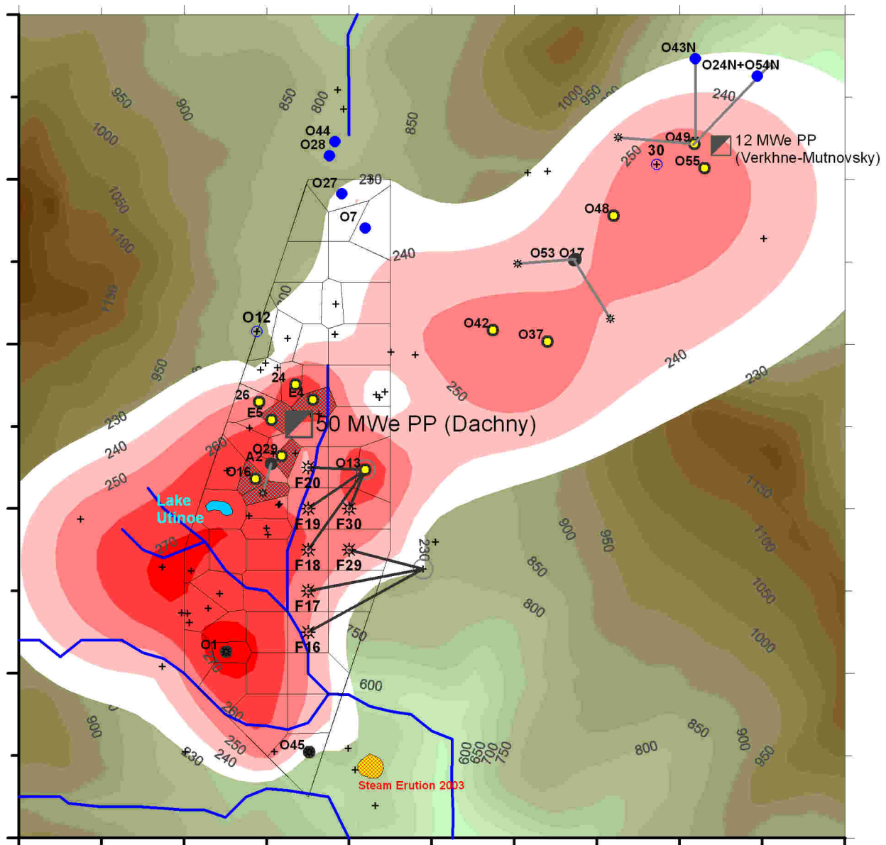
Figure 4: Schematic map of Mutnovsky geothermal field. Background contours are topography and temperature distribution at -250 m.a.s.l. Limits of this map correspond to limits numerical model (Kiryukhin, 1996); internal grid correspond to detailed model of the Main production zone (Kiryukhin et al, 2005, Kiryukhin and Vereina, 2005). Main exploitation wells - circles with yellow marks inside; reinjection wells - blue filled circles; monitoring wells - empty blue circles (30 and O12); directional wells - lines terminated at bottom positions (stars); small crosses - drillholes; hatched area – infiltration zone, assumed in modeling scenario EX3F; F-wells - additional production wells (F16, F17, F29, F18, F19, F20, F30) considered in the modeling scenario to provide Mutnovsky GeoPP 50 MW power with steam from the central block of Dachny site. Grid – 500 m
