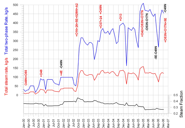
Figure 7: Mutnovsky geothermal field: observed total two-phase production rate (upper graph), observed total steam production rate (middle graph) and corresponding steam fraction (lower graph). Data from Maltseva et al, 2007
