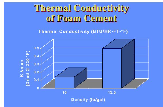
Figure 3: Thermal conductivity of foam cement vs. conventional cement.
