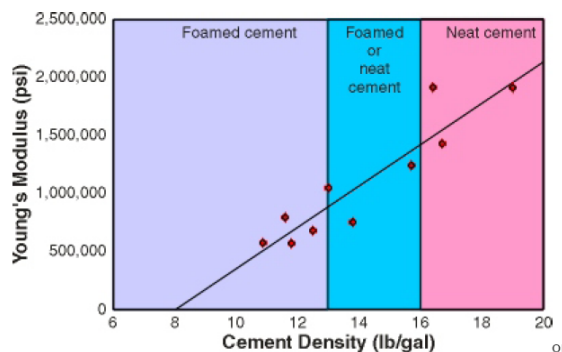
Figure 2: Young's Modulus at different densities and types of cement.
