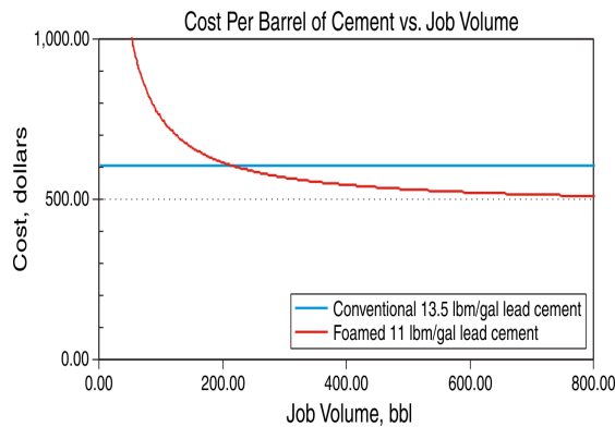
Figure 4: Cost per barrel of cement vs. job volume.
