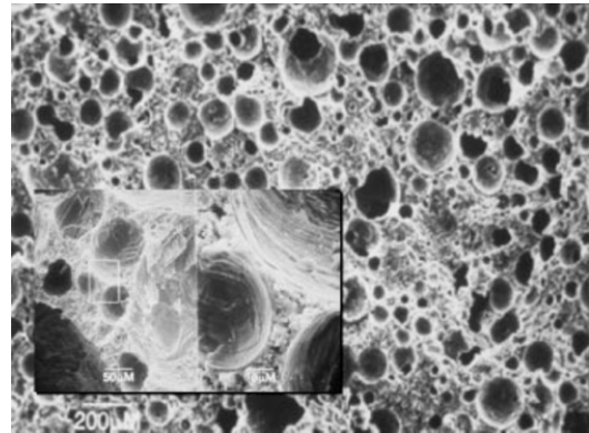
Figure 1: Microphotographs of a foamed cement sample.
