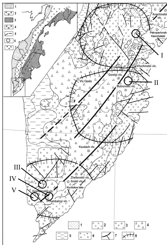
Figure 1: Geothermal Regions of South Kamchatka: the Structural Plan (Rychagov et al., 2006.). Inset map: main structural areas of Kamchatka in Paleogene-Neogene time (made by G.M.Vlasov and V.V. Yarmolyuk in 1964): 1 – West-Kamchatka, 2 – Central Kamchatka, 3 – East-Kamchatka; 4 – Sredinny massif (Sredinny Ridge); 5 – boundary of the East-Kamchatka volcanic zone; 6 – geothermal regions; 7 – geothermal systems. Main map: 1 – Pre-Island-Arc-Stage rocks (Pre-Oligocene); 2 – Lower structural stage (Oligocene (?)) – Middle Miocene); 3 – Middle stage (Middle Miocene-Pliocene); 4 – Upper stage – Quaternary volcanites; 5 – Quaternary and Pliocene - Quaternary (?) sedimentation masses of the upper structural stage of the internal area of the island arc; 6 – Large bodies of the quartz diorite complex; 7 – Faults; 8 – Boundary of geothermal areas, from North to South: Paratunsky, Mutnovsky-Zhirovsky and Pauzhetsky-Kabalny-Koshelevsky. Roman numbers indicate geothermal fields: I – Paratunsky, II – Mutnovsky, III – Pauzhetsky, V – Lower-Koshelevsky; and thermal manifestations of Kamalnyi Ridge (IV).
