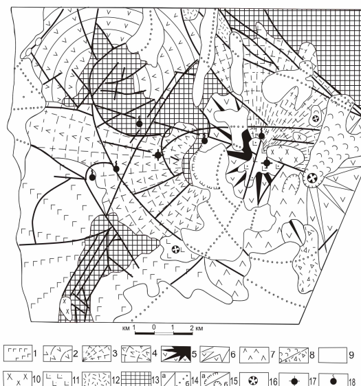
Figure 2. Geological plan of the Koshelevsky volcanic massif (Vakin et al., 1976; in authors modernization). 1, 2 – Lower-Quaternary volcanoes: 1 –Ded i Baba (Grandfather and Grandmother), 2 – Tret'ya Rechka (The Third River); 3-8 – effusive and pyroclastic formations of Koshelevsky massif: 3 – Drevniy Volcano (Ancient), 4 – Zapadnyy (Western), 5 – 1545 Volcano, 6 – Vostochniy (Eastern), 7 – Tsentralniy (Central), 8 – formations of the Active crater, a – lava flows, b – deposits of directional explosion; 9 – loose deposits of different age and genesis; 10 – extrusions of Holocene age; 11 – subvolcanic intrusions of dolerites; 12 – volcanic-sedimentary deposits of the Pauzhetsky suite; 13 – Pre-Quaternary effusive; 14 – discontinuous faults, a – identified, b – presumed; 15 – calderas (a) and erosion craters and explosion funnels (b); 16 – effusive and cinder cones; 17 – main thermal anomalies (the Upper-Koshelevsky confined to subvolcanic intrusion of dolerites and Lower-Koshelevsky – in the center); 18 – hot springs.
