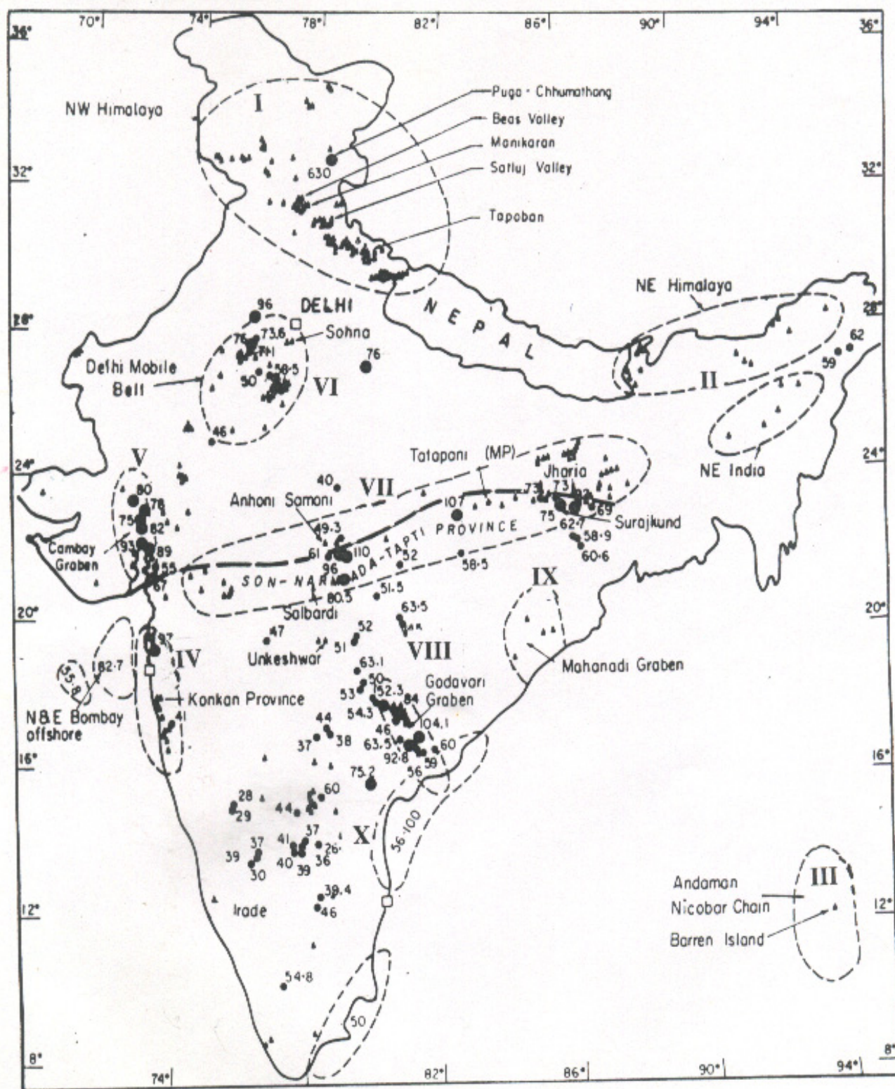
Figure 1: Geothermal provinces and regional flow pattern in India
