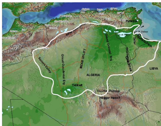
Figure 1: Map showing major basin features and approximate boundary of the NSAS
