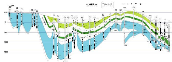
Figure 4: Geologic cross-section along the West (Algerian Atlas)-East (Libya) transect. Blue color shows the CI, White and green band shows the CT (OSS,2003)
