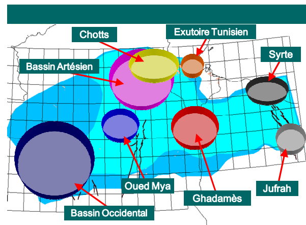
Figure 5: Critical areas of NSAS
