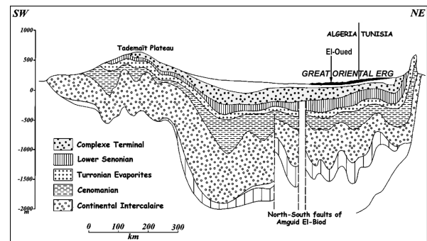
Figure 3: Geologic cross section along North Algeria-Tunisia transect
