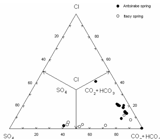
Figure 2: Relative Cl, SO 4 and CO 2 +HCO 3 contents of the Antsirabe-Itasy thermal waters on weight (mg/kg) basis. Fields from Giggenbach (1988).
