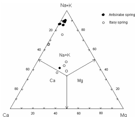
Figure 3: Relative Na+K, Ca and Mg concentrations.
