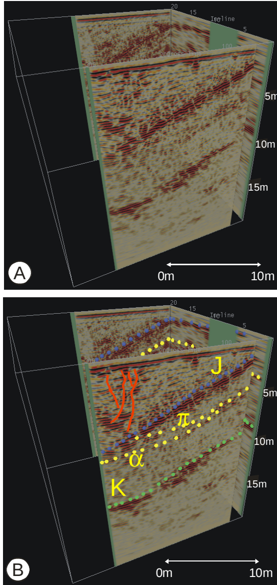
Figure 2: Example of 3-D multi-fold GPR data volume from the area of study (NE-Italy): A) in-line and cross-line selection (250 MHz data); B) interpreted data (stratigraphic joints as dotted lines, fractures as continuous red lines)
