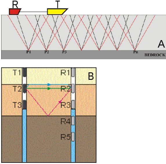
Figure 1: A) surface multi-fold ground-penetrating radar and B) cross-well tomography ground-penetrating radar data acquisition schemes used in the present work
