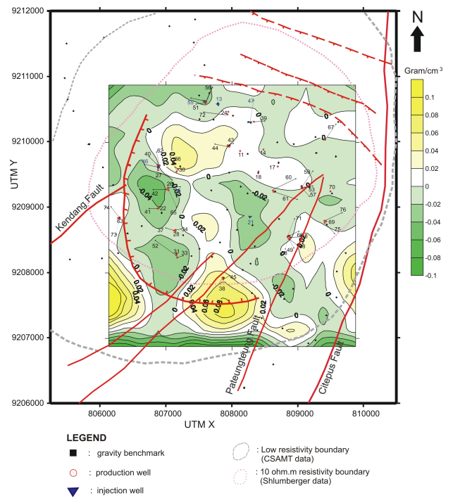
Figure 6: Density changes Jul'07-Jun'06 period at 1100 m depth
