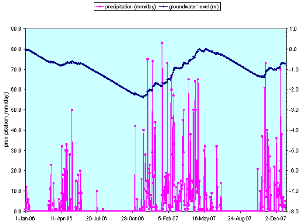
Figure 2: Groundwater level and precipitation
