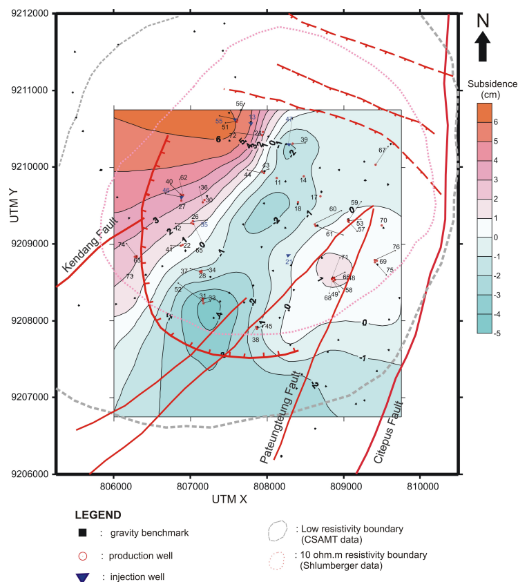
Figure:1 Subsidence rate in Kamojang 2006-2007
