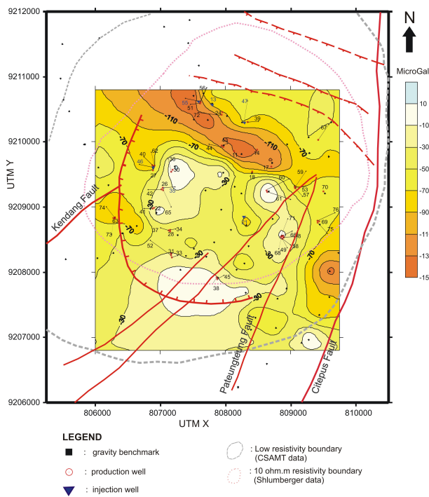
Figure 3: Gravity anomaly used stripping filter Jun'06-Nov'06 period
