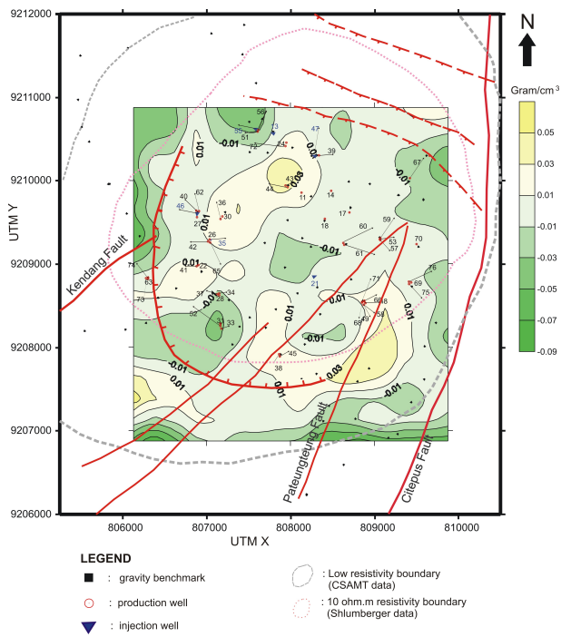
Figure 5: Density changes Jun'06-Nov'06 period at 1100 m depth
