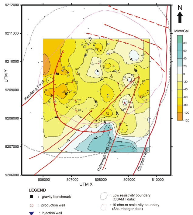
Figure 4: Gravity anomaly used stripping filter Jul'07-Jun'06 period
