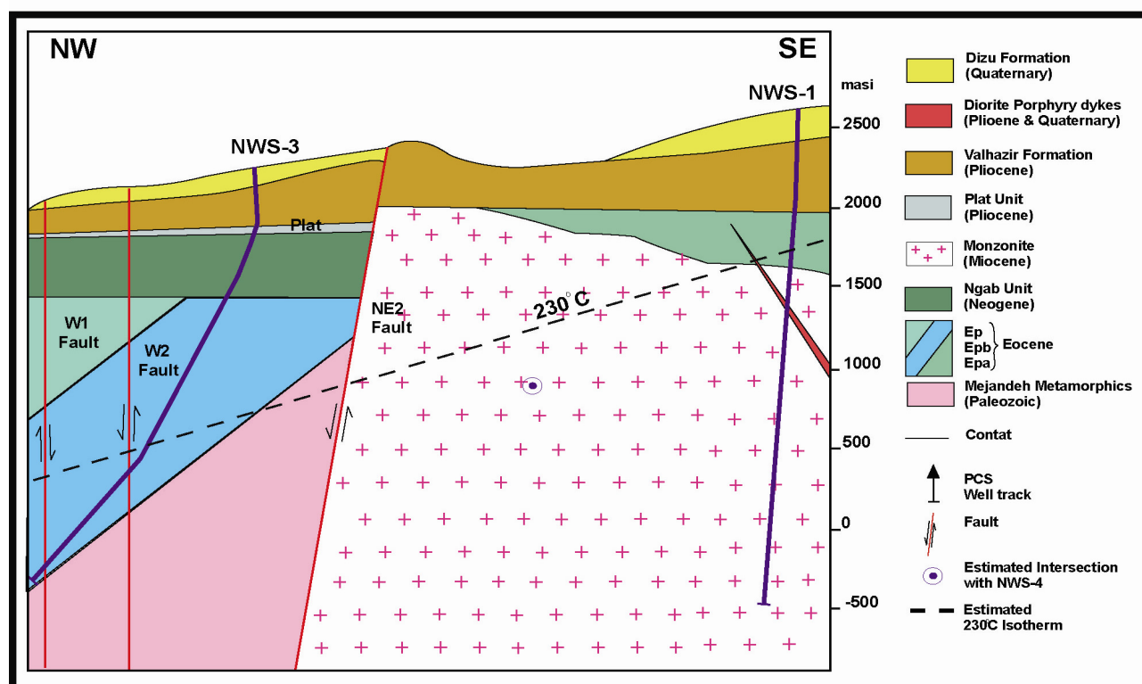
Figure 2: Geological Cross Section
