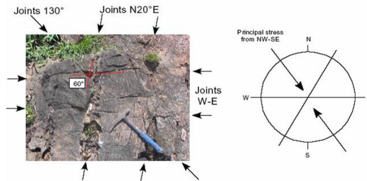
Figure 4. Joints in amphibolite outcrop. The main joints form a 60° angle, and the main stress field is from NW-SE as per stress diagram to the right. (After Gislason et al., 2004).
