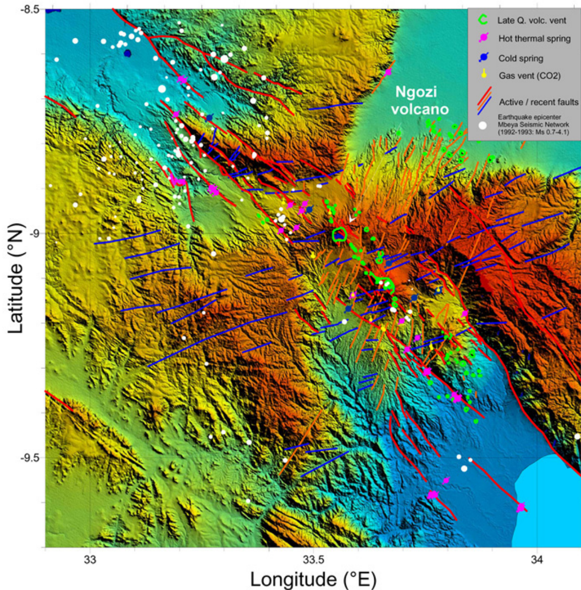
Figure 4: Evidence for recent tectonic activity: fault lines, earthquake epicentres (from Camelbeek and Iranga, 1996), recent volcanic vents (from Fontijn et al., submitted), and thermal springs differentiated as hot thermal (temperature above ambient, sometimes with CO 2 ), cold meteoric springs, and CO 2 vents with no water outflow.
