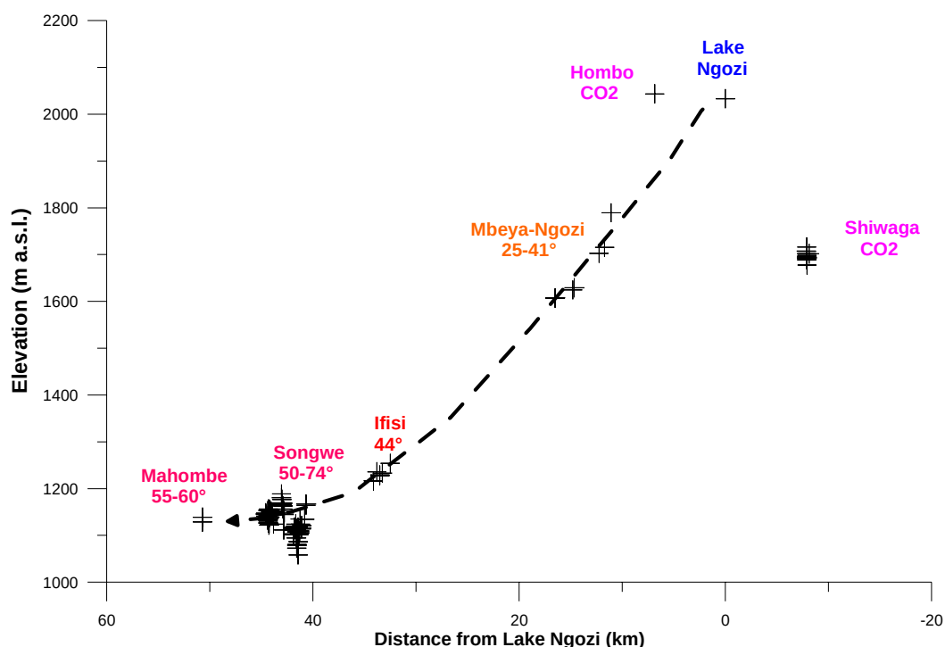
Figure 7: Distance – elevation plot of the thermal springs with their temperature, from the Ngozi volcano recharge area to the Songwe valley discharge.
