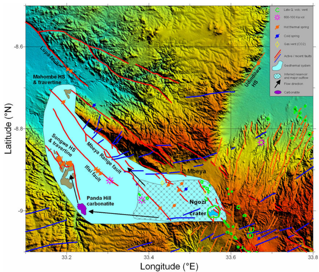
Figure 6: Map of the proposed Ngozi - Songwe Hydrothermal System.
