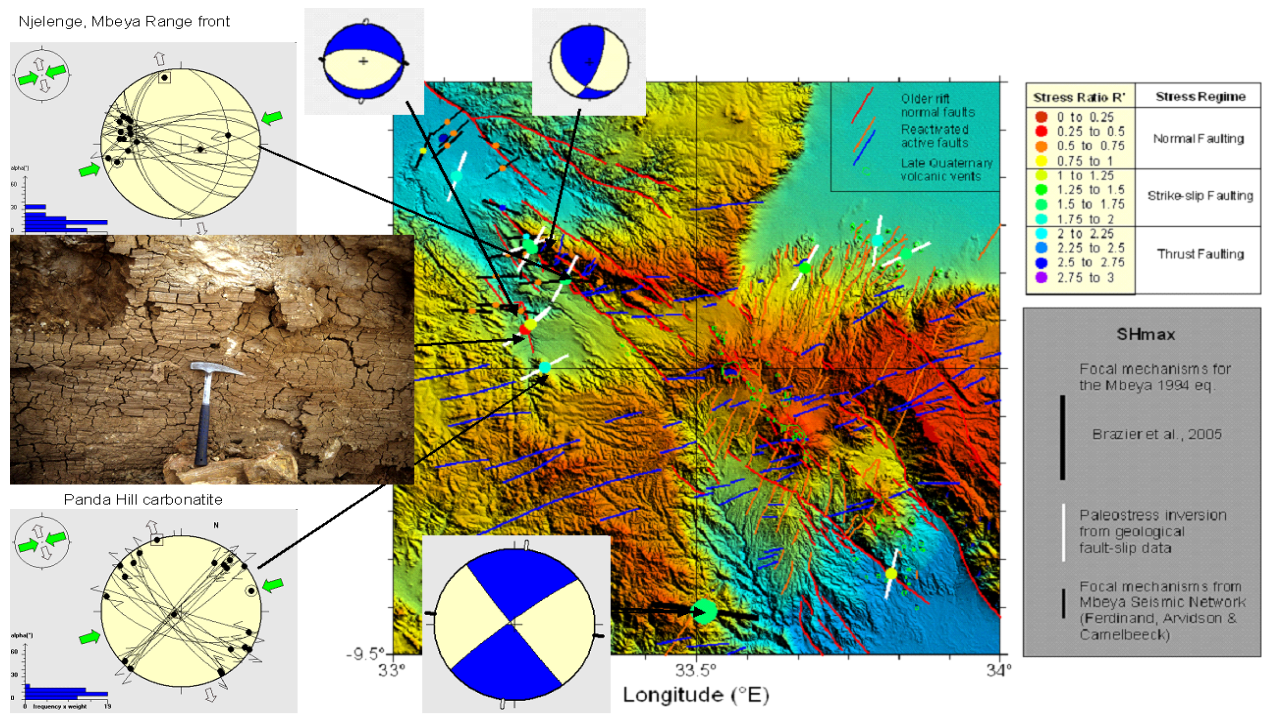
Figure 5: Tectonic stress in the Mbeya area, combining geological field data with earthquake focal mechanism data from Ferdinand and Arvidsson, (2002) and Brazier et al. (2005).
