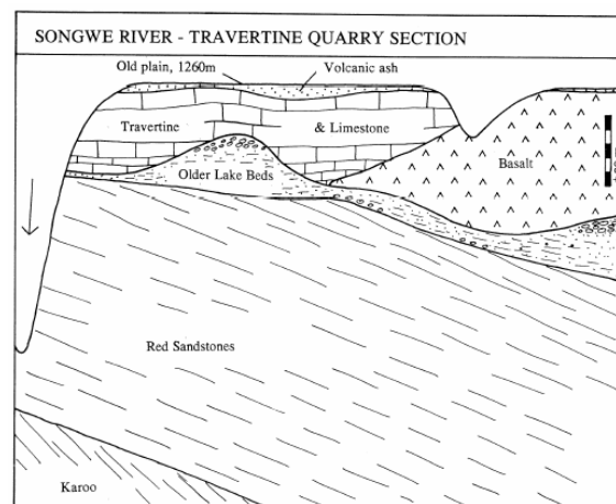
Figure 3: Stratigraphic succession in Songwe area including evidence from drill holes (from Delvaux et al. 1992)
