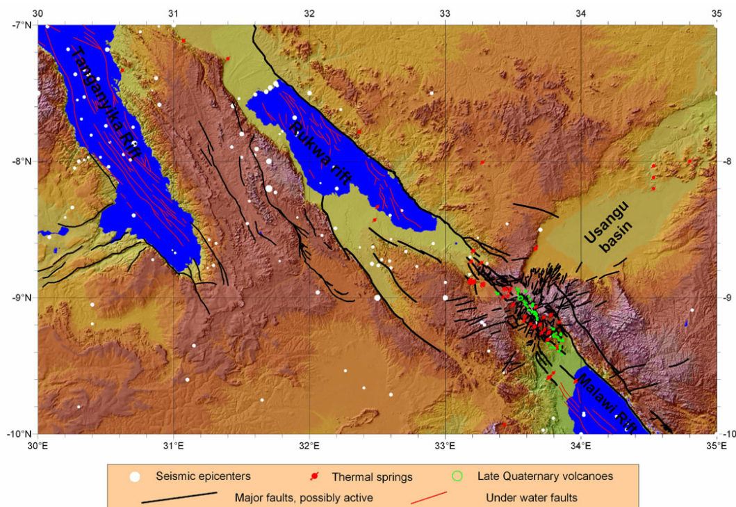
Figure 2: Neotectonic faults in the South Tanganyika – Rukwa – Nyasa region, with seismic epicenters, thermal springs and Quaternary volcanoes (after Fontijn et al., submitted) of the Rungwe Volcanic Province on the background of colour-coded SRTM DEM.
