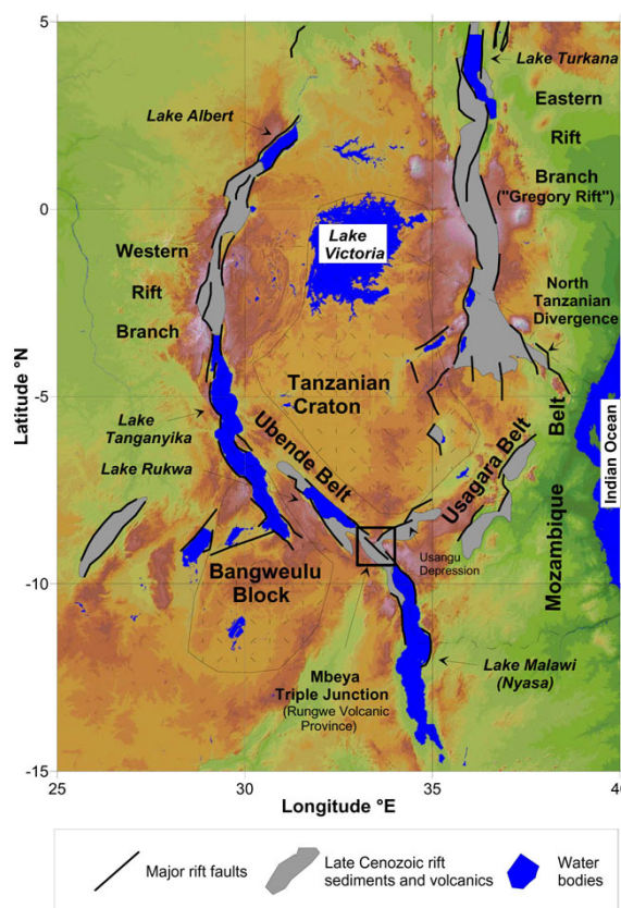
Figure 1: Location of the area regarding the Basement and the rift structure, on the background of colour-coded SRTM DEM.
