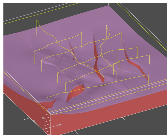
Figure 6: View to the NE of the model A, which is not satisfactory because of intra-block distortion. Violet Buntsandstein reservoir, red: crystalline basement (30 km on E-W axis and 32 km on N-S axis).
