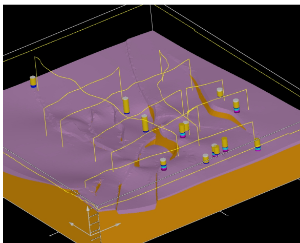
Figure 7: View to the NE of the acceptable model B. Violet: Buntsandstein reservoir, orange: crystalline basement. The cylinders represent the boreholes (30km on E-W axis and 32km on N-S axis).
