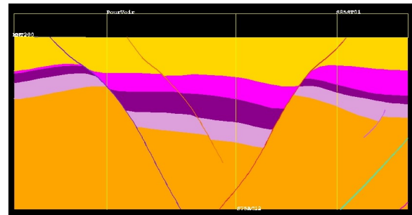
Figure 5: Example of interpolated interfaces and faults in a seismic cross-section (75AC2 profile). Yellow: Tertiary, pink: Jurassic and upper Trias, purple: Muschelkalk, violet: Buntsandstein, orange: granitic basement (total cross-section length: 12.5 km).
