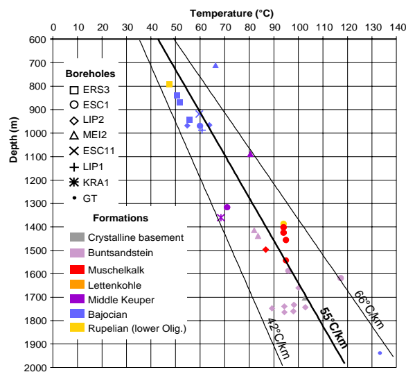
Figure 4: Temperatures in the previous oil boreholes and calculated geothermal gradient. Location of boreholes: Figure 2.
