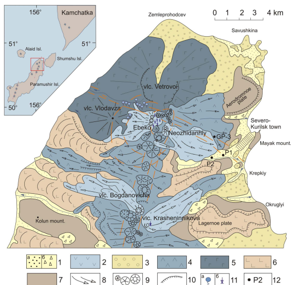
Figure 2: The schematic geological map of the northern part of Paramushir Island (Present-Hydrothermal..., 1998). 1 – present alluvial, marine and lacustrine strata (a) and talus (b); 2 – andesitic, andesibasaltic lavas ( Q_4 ); 3 – glacial deposits ( Q_3^4 ); 4 – andesitic lavas ( Q_3 ); 5 – andesitic, andesibasaltic lavas ( N_2^2 - Q_1 ); 6 – basaltic lavas, tuffs, tuff-breccias ( Q_{1-2} ); 7 – undivided volcano-sedimental deposits and subvolcanic bodies ( N_1^3 - N_2 ); 8 - centers of volcanic eruptions; 9 – small volcanoes, lava and cinder cones located in axial zone of the Vernadsky ridge; 10 – displayed in the relief scarps and erosional limits of calderas; 11 – thermal springs (a) and fumaroles (b); 12 – drill holes.
