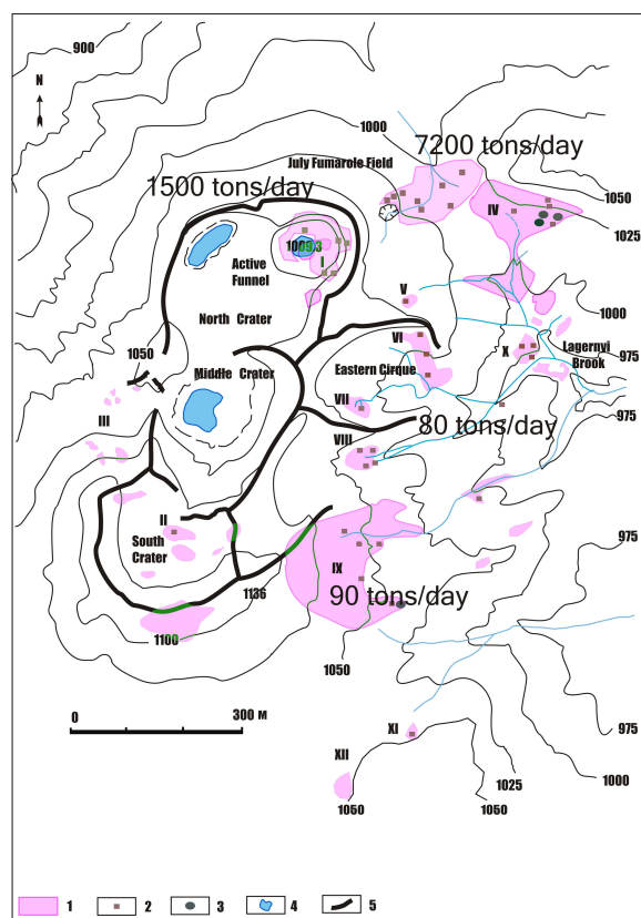
Figure 3: The crater zone of Ebeko volcano. 1- Map of Ebeko volcano thermal fields, after V.N. Dvigalo (1989) and supplemented by these authors: (1) thermal fields, (2) fumaroles, (3) pots of thermal water, (4) crater lakes, (5) rims of major craters. Roman numerals denote thermal fields: (I) Active Funnel, (II) South Crater, (III) West Field, (IV) Northeastern Field, (V) Gremuchaya fumarole field, (VI) Florenskii fumarole field, (VII) First Eastern Field, (VIII) Second Eastern Field, (IX) Southeastern Field, (X) Lagernyi Brook field, (XI) Second Southeastern Field, (XII) Third Southeastern Field. 90 tons/day and so on – it is the quantity of steam, allocated by fumaroles on the basic thermal fields.
