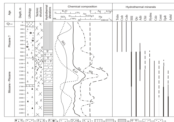
Figure 6: Deep geological-geochemical cross section of Severo(North)-Paramushirsky Hydrothermal-Magmatic System and North-Kurilsky geothermal deposit (well GP-3). 1 – lithocrystalloclastic intrusive tuffs of andesibasaltic; 2 – andesite lavas; 3 – multicoloured lithoclastic tuffs of andesite; 4 – tuffites with inclusions of a relic organic material; 5 – andesibasaltic lavas; 6 – tectonic and other breccias; 7 – cracks; 8 – low-temperature opal-cristobalite-tridymite-chalcedony metasomatites; 9 – low-middle-temperature quartz-adularia-hydromica metasomatites; 10 – middle-temperature quartz-chlorite-epidote-muscovite propylites; 11 – vapor-dominated zones (quartz-adularia metasomatites); 12 – quartz-chalcedonic veins with ore minerals; 13 – ore mineralization.
