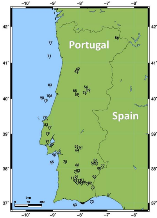
Figure 3: Heat flow density map for mainland Portugal. Values are in \text{mW/m}^2 .
