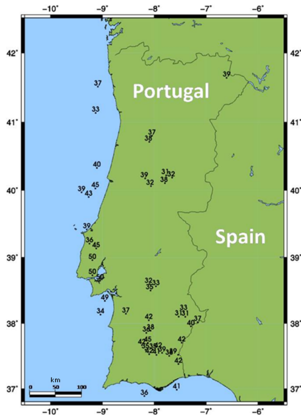
Figure 5: Temperature at 1000 m depth for mainland Portugal. Values are in °C.
