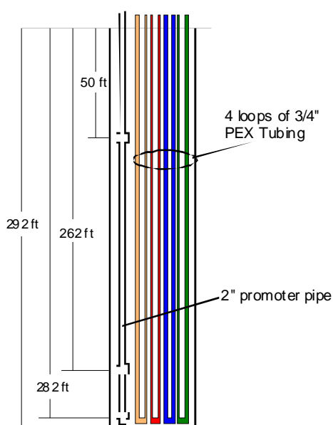
Figure 6: Schematic of System One well
