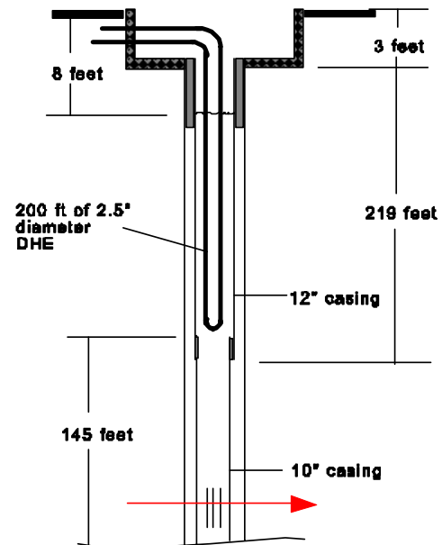
Figure 10: Schematic of System Three well
