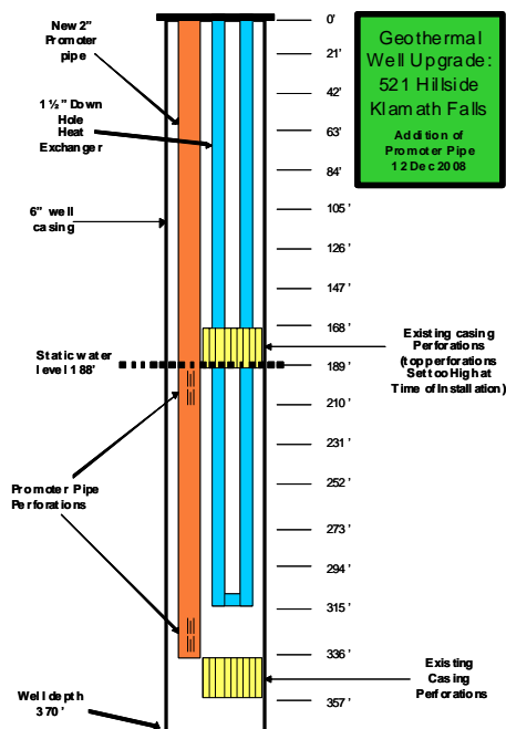
Figure 9: Schematic of System Two well
