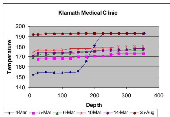
Figure 12: Temperature vs. depth profile of System Three well before and after the operation of the promoter pipe
