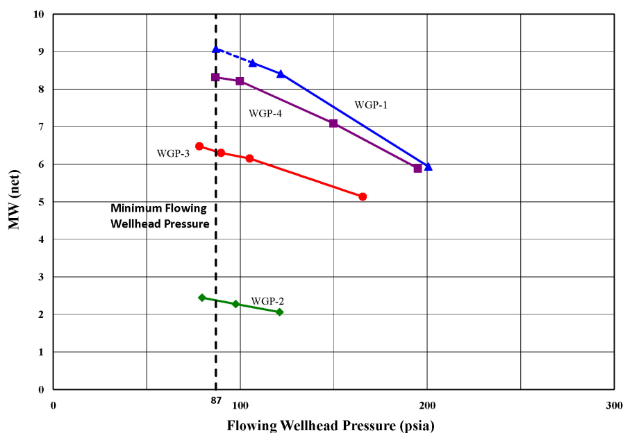
Figure 10: Western GeoPower Unit 1 Well Test Results
