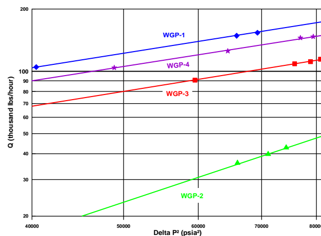
Figure 9: Well Deliverability Plots
