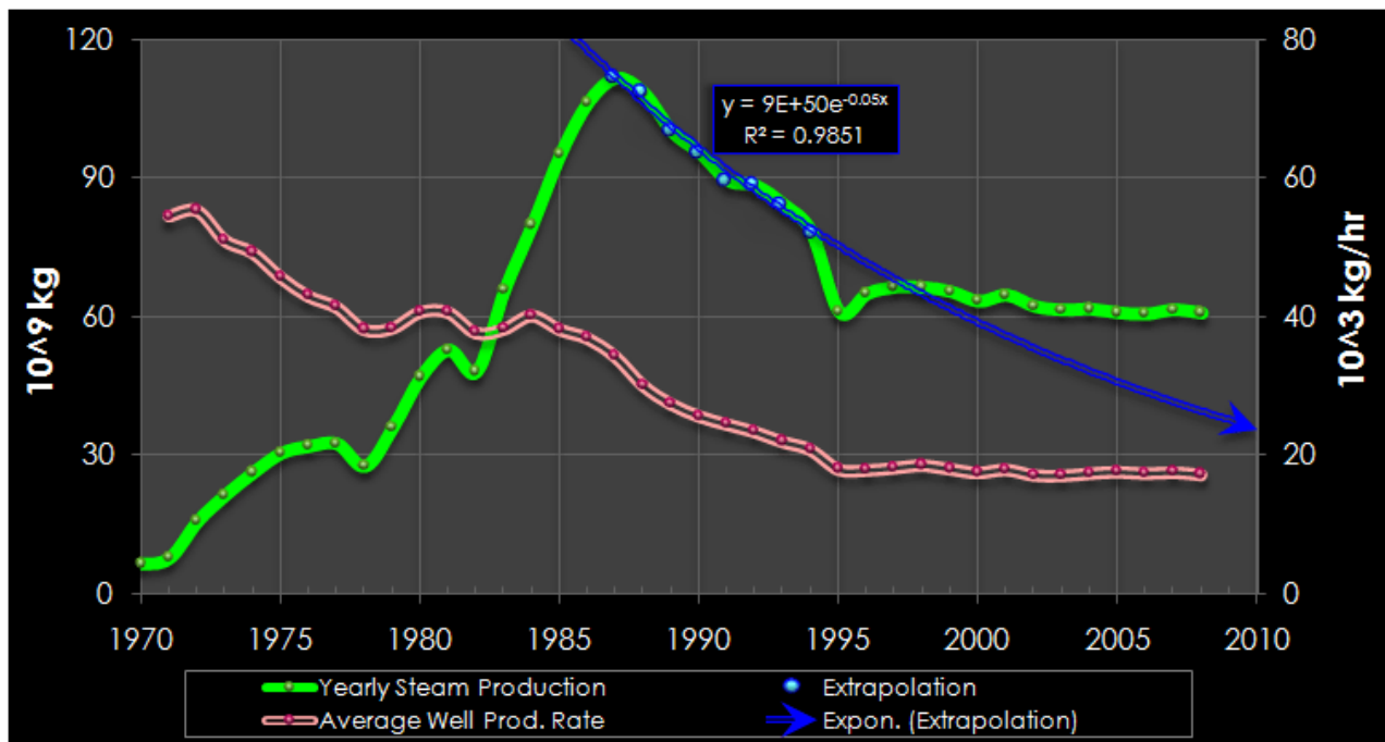
Figure 1: Yearly Field-wide Steam Production and Average Well Production/Month (Source: Division of Oil, Gas, and Geothermal Resources).
