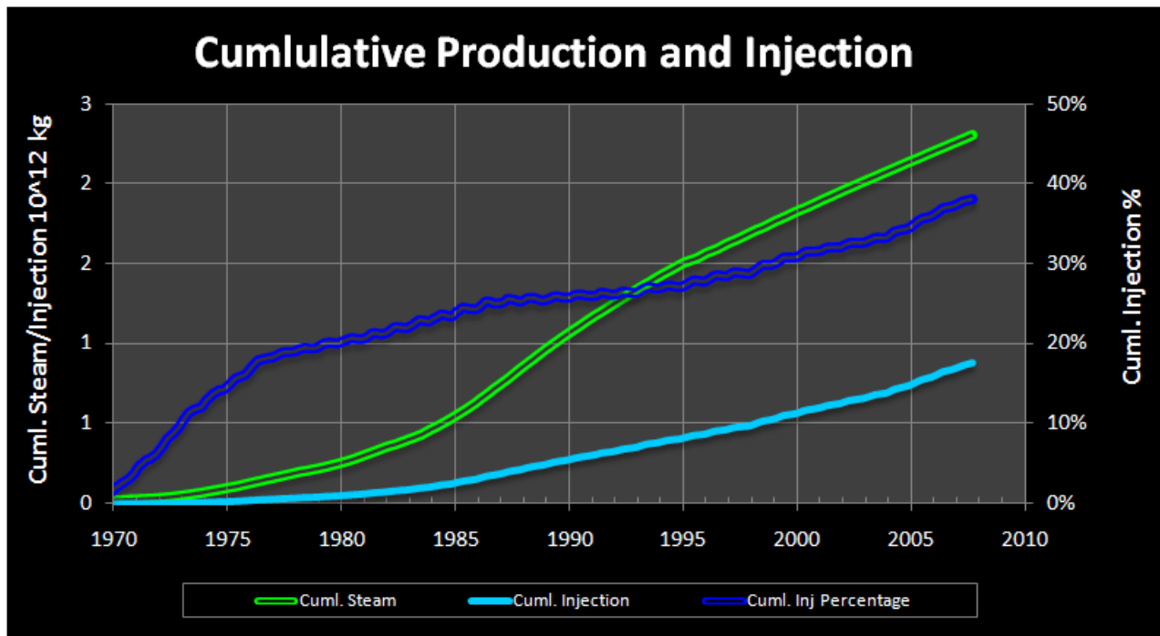
Figure 3: The Geysers had produced 2,394 billion kg of steam and injected 946 billion kg of fluids, resulting in a lifetime net mass replacement of 39.5% (Source: Division of Oil, Gas, and Geothermal Resources).
