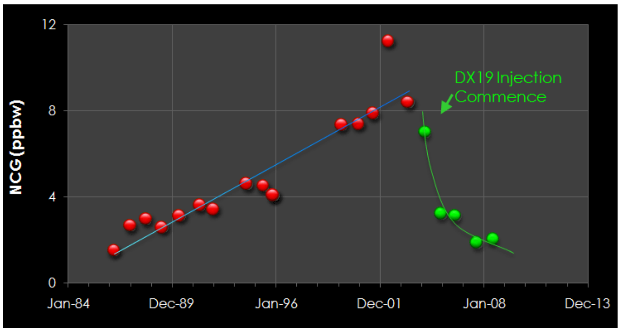
Figure 4: NCG concentration versus time in well DX85 (Courtesy of Calpine).
