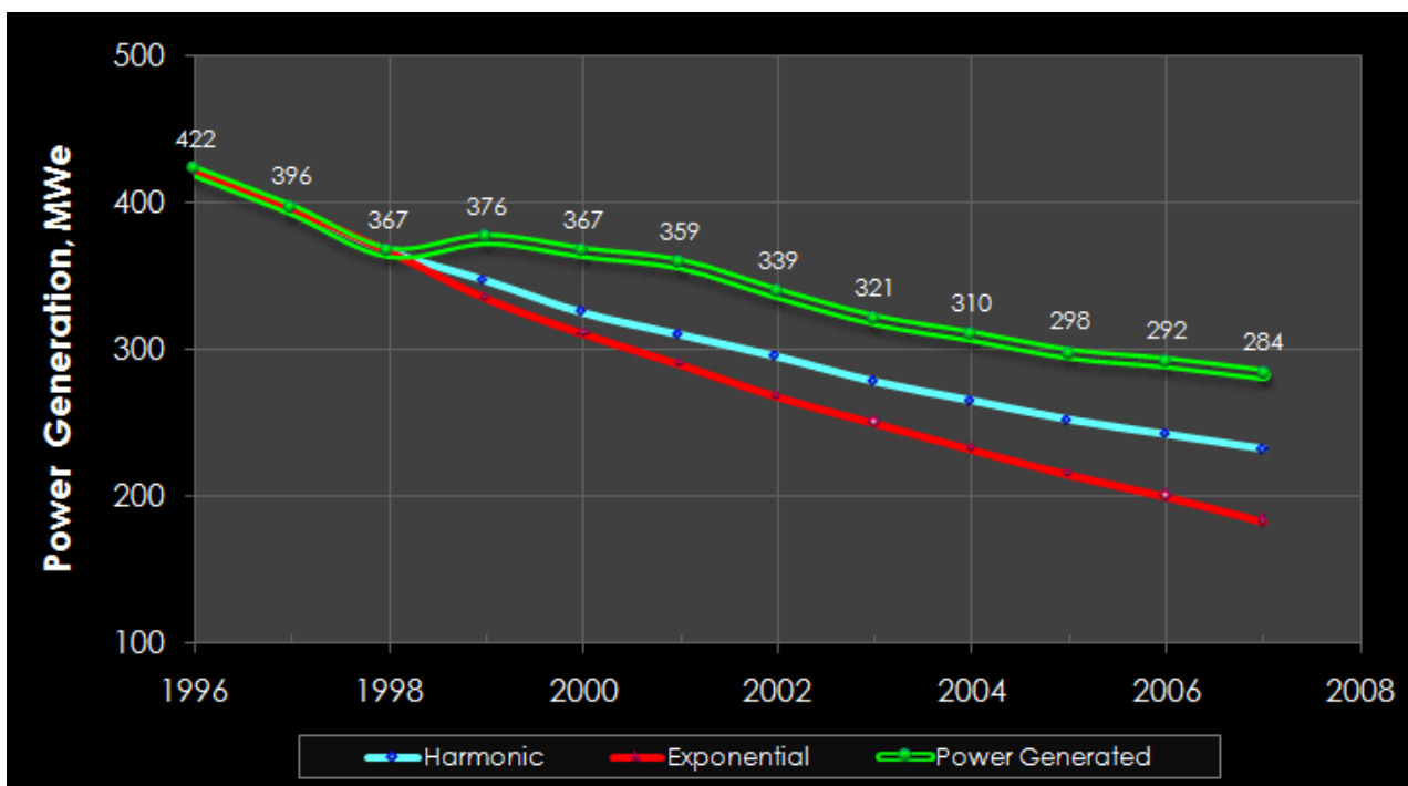
Figure 2: Effect of SEGEP Injection on Southeast Geysers (Courtesy of Calpine and NCPA).
