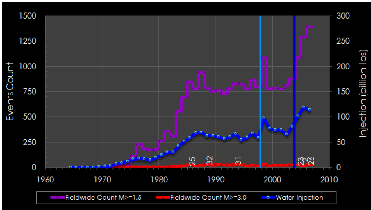
Figure 5: Seismicity and Injection in Southeast Geysers (Courtesy of Calpine).
