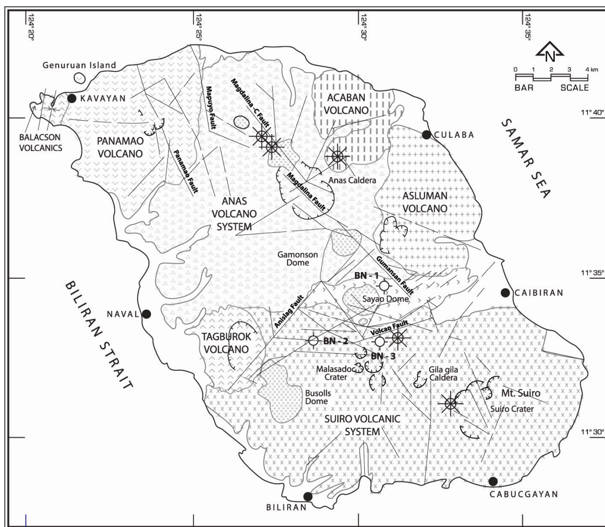
Figure 3: Simplified Geological Map of Biliran
