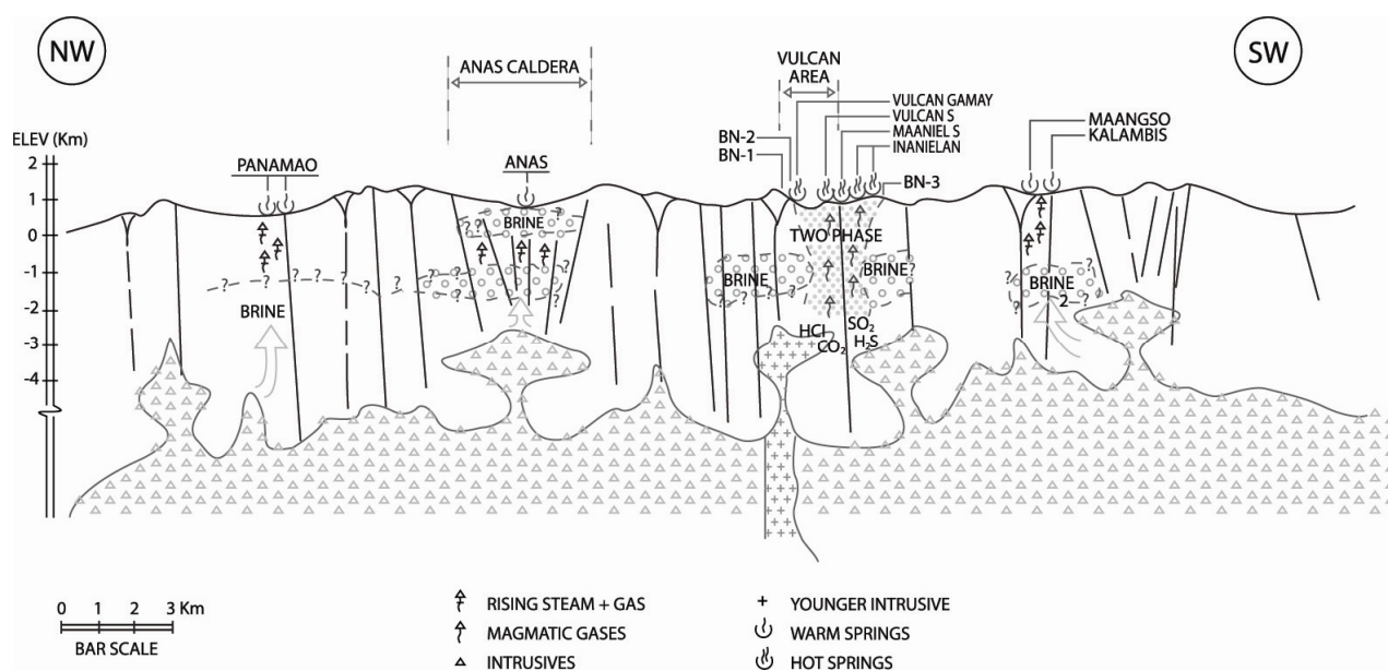
Figure 1: Different Hydrothermal Systems in Biliran
