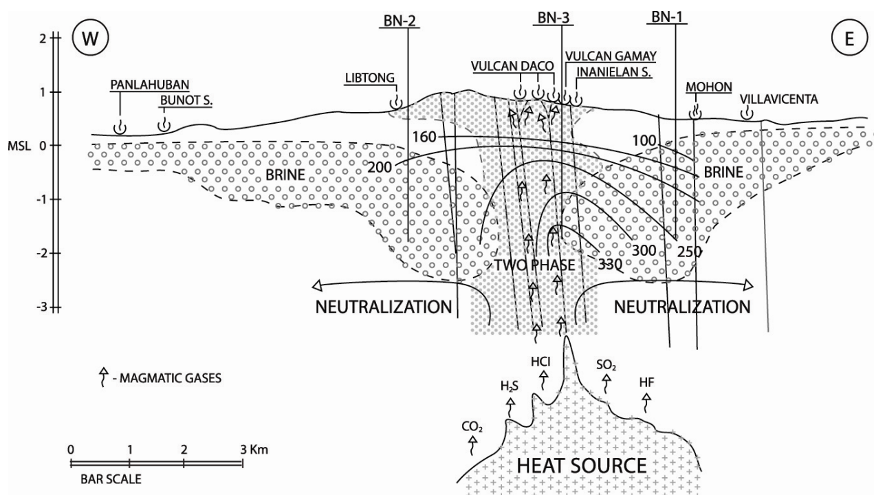
Figure 2: The Geothermal Model of the Vulcan-Libtong Area
